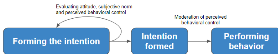
Figure 8. Proposed automaton
