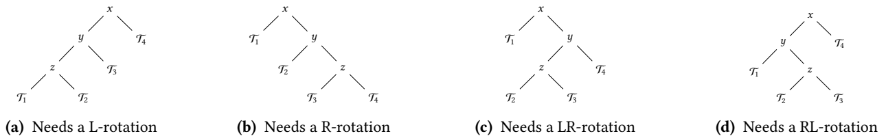
Figure 2. Unbalanced trees
