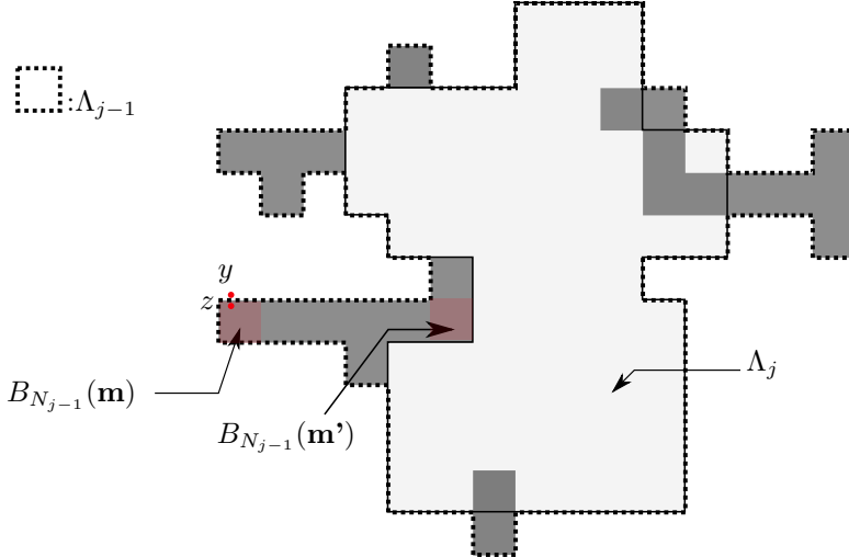
Figure 2 – Representation of y, z and \mathbf{m}, \mathbf{m}'
