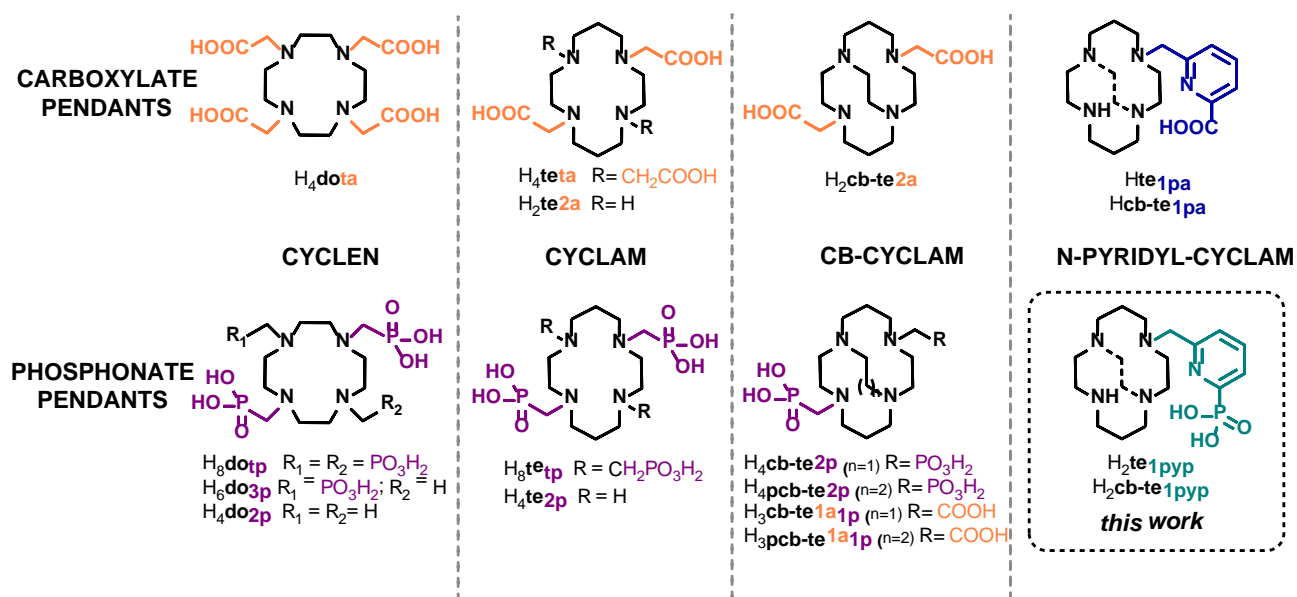
Figure 1 : Copper(II) chelators discussed in this paper
