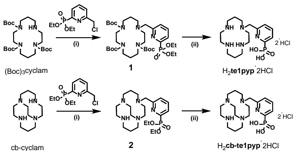
Scheme 1: Synthetic protocol for the preparation of the ligands; H 2 te1pyp and H 2 cb-te1pyp ; (i) K 2 CO 3 , MeCN, RT, 36 hr ( 1 58%; 2 ·HCl 84%) (ii) 6 M HCl (aq) , 100°C, 36 hr ( H 2 te1pyp 89%; H 2 cb-te1pyp 60%)
