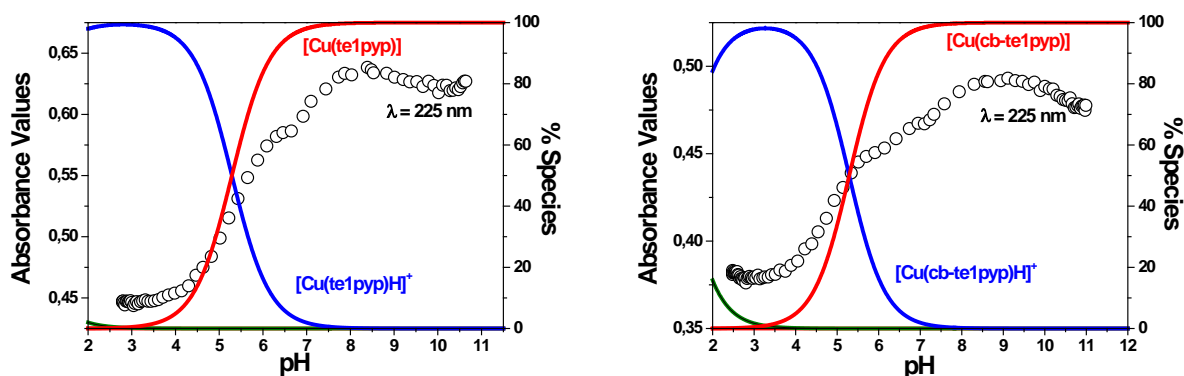
Figure X. Distribution diagrams of the cupric complexes with te1pyp and cb-te1pyp in solution (from potentiometric data) as a function of pH, compared to the variation of the absorbance at 225 nm as a function of the pH. To compare the coordination properties of te1pyp and cb-te1pyp with other copper(II) chelators, their pCu values ( Table 4 ) were calculated at pH = 7.4. 55,62 These pCu values measure the equilibrium concentrations of free Cu^{2+} ion and are defined as: pCu = -\log [Cu^{2+}]_{free} with [L]_{tot} = 10^{-5} M, [Cu^{2+}]_{tot} = 10^{-6} M. This pCu value takes into account the characteristics of the ligands that are compared (acido-basic properties of the free ligand and of the metal complexes, stoichiometry of metal complexes, etc) and thus allows a direct comparison of their chelating affinity for a given cation. High pCu values will therefore be a signature of a strong binding affinity of the chelator toward Cu^{2+} . For te1pyp and
