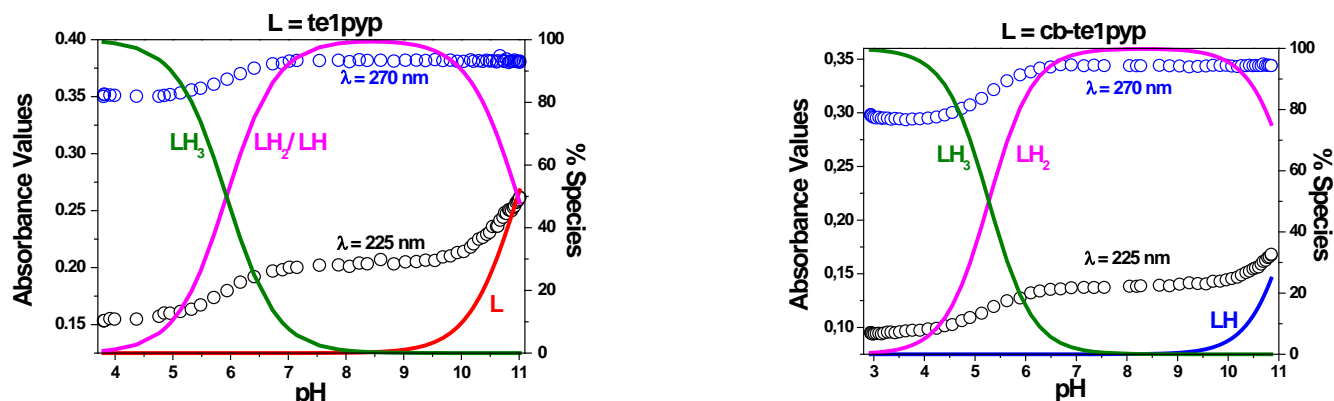
Figure X. Distribution diagrams of the protonated species of te1pyp (left) and cb-te1pyp (right) in solution. Top : from potentiometry; bottom : from absorption versus pH data, compared to the variation of the absorbance at 270 nm and 225 nm as a function of the pH.
