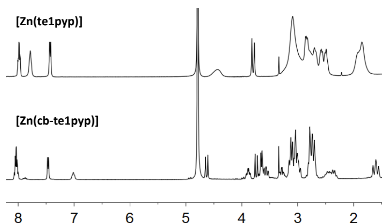
Figure X: ^1H NMR spectra ( D_2O , pD \approx 7.0 , 400 MHz, 298 K) of zinc(II) complexes [Zn(te1pyp)] and [Zn(cb-te1pyp)]
