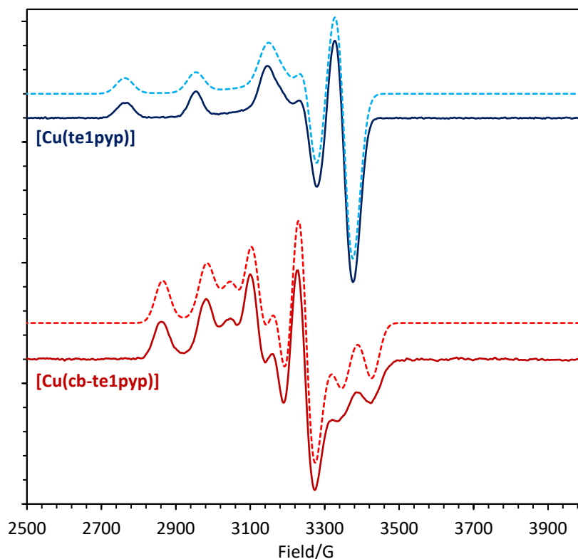
Figure X: X-band EPR spectrum of copper(II) complexes [Cu(te1pyp)] (— experimental; - - - simulation) and [Cu(cb-te1pyp)] (— experimental; - - - simulation) recorded in frozen aqueous solution (1:1 DMF/H 2 O, 1.0 mM; 150K)
