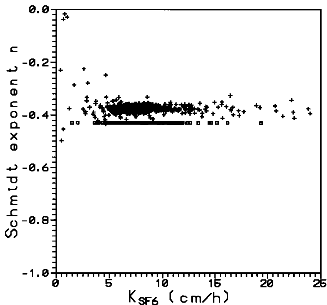
Figure 14. Variation of the Schmidt number exponent versus K_{SF_6} using selected pairs on the \delta^3\text{He}(t) and \text{SF}_6(t) best fit curves computed with the well-mixed box model (open squares) and the vertical diffusion model (crosses).
