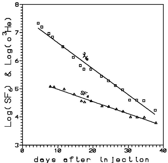
Figure 4. Logarithm of the tracers' concentrations (SF 6 and δ 3 He‰) versus time
