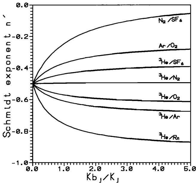
Figure 15. Theoretical variation of the apparent Schmidt number exponent n' versus K_{b_j}/K_j derived from equation (8) for various inert gas pairs ( i,j ). The K_{b_i}/K_{b_j} ratios have been computed assuming that K_b varies with the gas solubility and diffusivity as (\text{SRT})^{0.3} D^{0.35} (where SRT is the Ostwald solubility coefficient) [Keeling, 1993]. Gas solubilities and diffusivities are computed using the polynomial fit of Wanninkhof [1992] for freshwater at 8°C.
