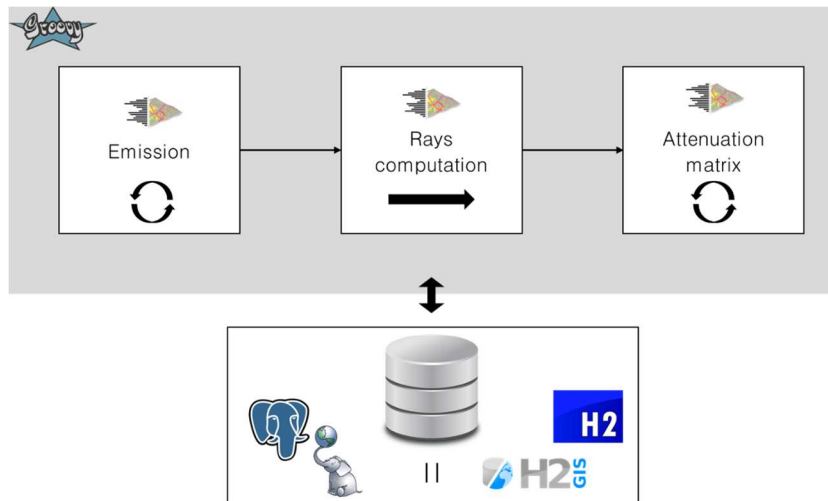
180 Figure 1 – Sensitivity analysis framework using NoiseModelling. The NoiseModelling JAVA libraries 181 directly interact with Postgre/PostGIS or H2/H2Gis databases.
