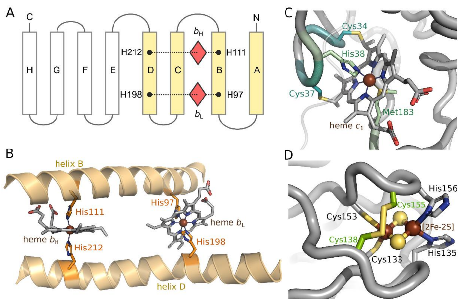
Figure 8. Structural features and binding motifs of metallic cofactors of Cyt bc_1 . A) Schematic representation of the transmembrane part of Cyt b , showing helices involved in formation of the heme-bearing 4-helix bundle (A-D, pale orange rectangles). Hemes are shown as orange polyhedrons, positions of axial ligands of hemes are marked by black dots, R. capsulatus residue numbering is used. B) Structural model showing hemes b orientation within the transmembrane bundle and orientation of their axial ligands. Helices providing axial ligands are shown in pale orange cartoon, ligating histidines are colored orange. C) Structural model showing heme c_1 binding site in the globular domain of Cyt c_1 . Cysteines of the binding motif are colored light blue, axial ligands are colored pale green. D) Structural model showing the [2Fe-2S] cluster binding site in ISP. Coordinating residues are labeled in black, cysteines that form the disulfide bridge are colored and labeled in green. All representations are based on PDB 1ZRT entry.
