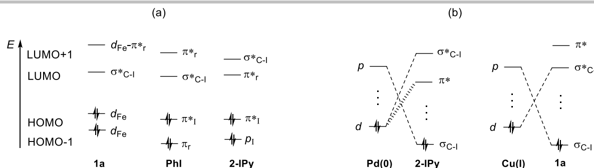
Scheme 2. (a) FMO profile of the selected species; (b) schematic representation of the allowed interactions between 2-iodopyridine (2-IPy) and Pd(0) [24] vs those of ferrocene (1a) and Cu(I).
