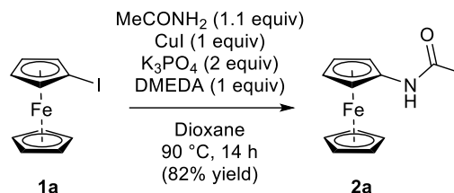
Scheme 1. N -arylation of acetamide with iodoferrocene.
