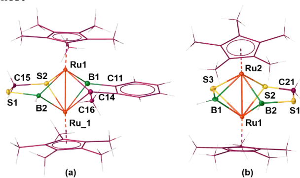
Figure 1. Molecular structure and labelling diagram of 2 (a) and 4 (b): Selected bond lengths (Å) and angles ( ^\circ ) are: 2 : C16-C14 1.526(19), B1-C11 1.575(19), C15-S1 1.73(2), C15-S2
