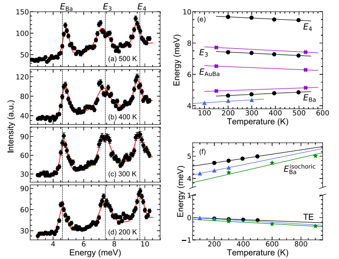
FIG. 7. (a)–(d) Inelastic neutron scattering (INS) intensity for constant \mathbf{Q} = (113) scans as a function of energy (black circles) recorded on IN12@ILL between 200–500 K for \text{Ba}_{7.81}\text{Ge}_{40.67}\text{Au}_{5.33} . The solid red lines are Gaussian fits of the three optical bands whose energies are referred to as E_{\text{Ba}} and E_{3,4} . The vertical dotted black lines indicate their values at 200 K. (e) Temperature dependence of E_{\text{Ba}} and E_{3,4} obtained from the fits shown in panels (a)–(d) (black circles) and from the E_{\text{Ba,Au}} and E_3 peaks in the generalized vibrational density of states shown in Fig. 3(c) (purple crosses). Blue triangles show the temperature dependence of E_{\text{Ba}} in \text{Ba}_8\text{Ge}_{30}\text{Ga}_{16} [59]. In (f), the temperature dependence of E_{\text{Ba}} for \text{Ba}_{7.81}\text{Ge}_{40.67}\text{Au}_{5.33} (black circles) and \text{Ba}_8\text{Ge}_{30}\text{Ga}_{16} (blue triangles), corrected for the thermal expansion (TE), are shown and compared to that of the \text{Ba}_8\text{Ge}_{30}\text{Ga}_{16} self-consistent phonon theory calculation that includes cubic and quartic terms (SCPB) [43] (green stars). The rates of TE of \text{Ba}_{7.81}\text{Ge}_{40.67}\text{Au}_{5.33} and \text{Ba}_8\text{Ge}_{30}\text{Ga}_{16} by INS and SCPB (same symbols/colors) are also plotted.
