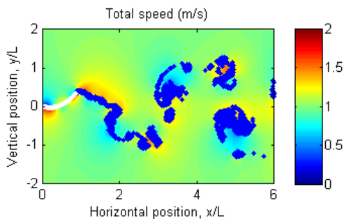
Fig. 13. Instantaneous flow velocity magnitude in the wake.
