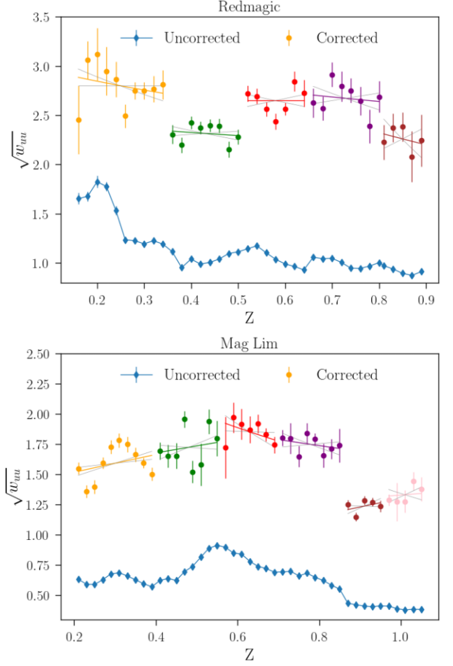
Figure 10. Autocorrelations of the DES lens samples, redMaGiC and MagLim. We show the square root of the autocorrelation, \sqrt{\bar{w}_{\text{uu,pz}}(z_j)} , listed as uncorrected. The corrected data points are \sqrt{\bar{w}_{\text{uu,pz}}(z_j)\sigma_j} , to undo the influence of photo- z scatter on the autocorrelations. The 11 different tomographic bins are differentiated by colour. The solid lines in colour are the best power-law fit to the points in a given bin (equation 12). The grey lines indicate the 1\sigma range of the power-law fit. We note that, because of the normalization of n(z) , the amplitudes of these measurements are not important, only the change across a single tomographic bin
