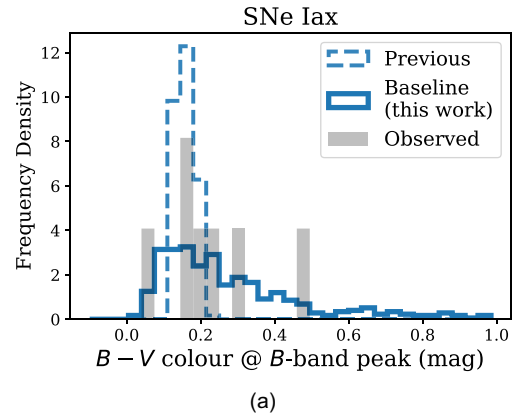
Figure 5. B - V colour distribution at B -band peak for SNe Iax simulated using the original PLAsTiCC models (dashed histogram), for the updated SNe Iax model used in this analysis (solid histogram; Section 4.3), and for seven observed SNe Iax for which good B - and V -band photometry around peak has been published (grey-filled histogram, SN 2003gq, SN 2005cc, SN 2005hk, SN 2008A, SN 2008ha, SN 2011ay, and SN 2012Z from Silverman et al. 2012; Foley et al. 2013; Stahl et al. 2019).
