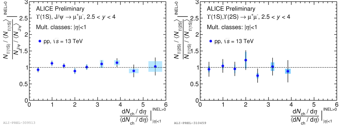
Figure 4: Left: Double yield ratio of Y(1S) over J/\psi as a function of normalized charged-particle multiplicity; Right: Double yield ratio of Y(2S) over Y(1S) as a function of normalized charged-particle multiplicity.
