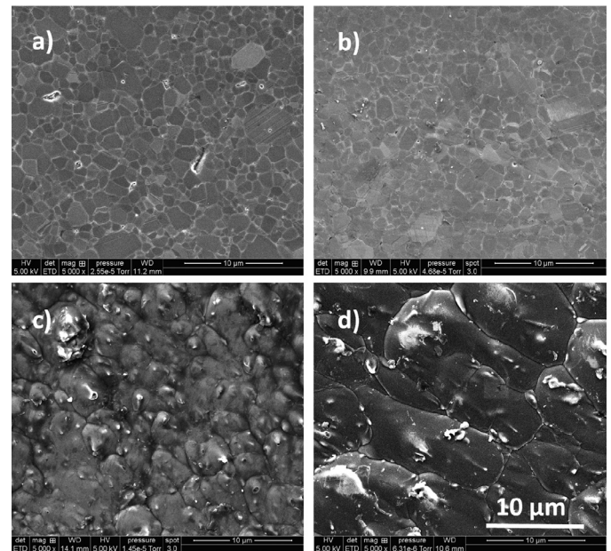
Fig. 2. SEM images of the \text{B}_4\text{C} sample surface before irradiation (a), after irradiation with 100 MeV sulfur ions at a fluence of 5 \times 10^{15} ions·cm ^{-2} (b), 60 MeV and 100 MeV iodine ions at a fluence of 3 \times 10^{15} ions·cm ^{-2} and 5 \times 10^{15} ions·cm ^{-2} respectively (c) and (d).
