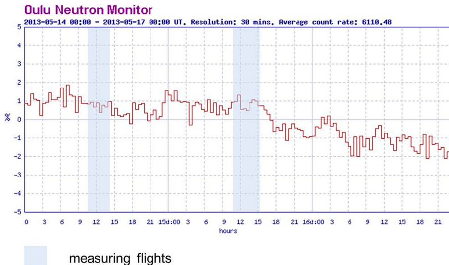
Fig. 2. Variation of the count rates of the Oulu neutron monitor during the measuring flights over South Germany and South Norway on the 14th and 15th May 2013 ( http://cosmicrays oulu.fi/ ). The corresponding W -parameter was 66 for each flight position (rounded, see Table 1).
