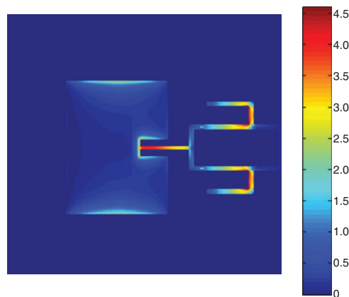
Fig. 2 Current distribution (A/m) at 2.45 GHz
