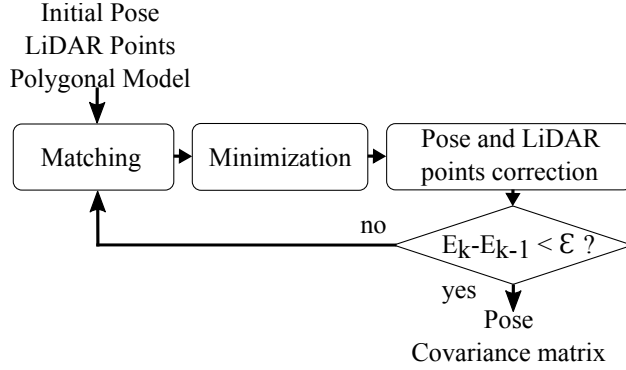
Figure 4: Iterative matching and minimization algorithm.
