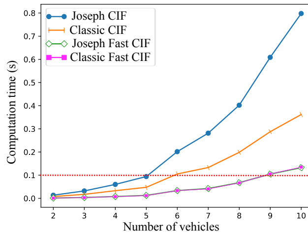
Figure 14: Classic and Joseph CIF and their fast implementations. Computation times for two to ten vehicles with the 10 Hz limit (in red). The pink and green curves are very close to each other.
