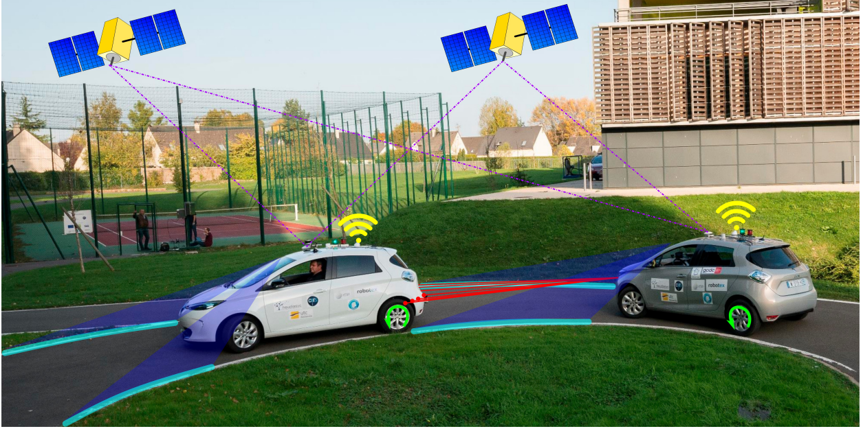
Figure 9: Platooning of two autonomous Renault ZOE's on the UTC Seville test track. Both vehicles use GNSS localization from a ublox 8 receiver (in purple). Direct Wifi 802.11p communication (in yellow) is simulated in this work, as is the detection of lane markings (in blue). The longitudinal speed and yaw rate (in green) are obtained from the CAN bus. Finally, the tracking vehicle is equipped with a SICK LD-MRS LiDAR (in red).
