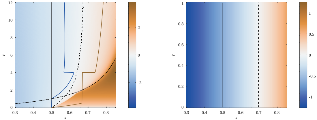
(C) Same as 3a with two colored lines delimiting a central zone where the sign is analytically unknown (cf. Theorems 1.1 and 1.2).
