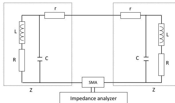
Figure 4. Electric diagram of the textile NFC combiner connected to an impedance analyzer.
