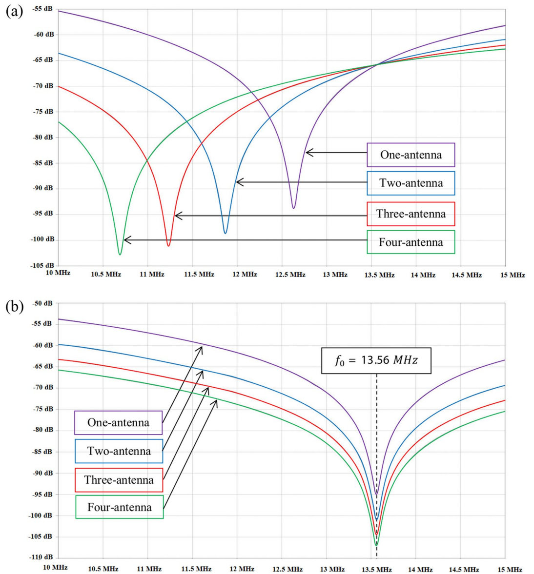
Figure 3. Simulated current in the branch of the impedance analyzer in dBA of the textile NFC combiners versus the frequency. (a) Current without taking into account C_{SMA} . (b) Current with taking into account C_{SMA} ( C' = C - N.C_{SMA} ).
