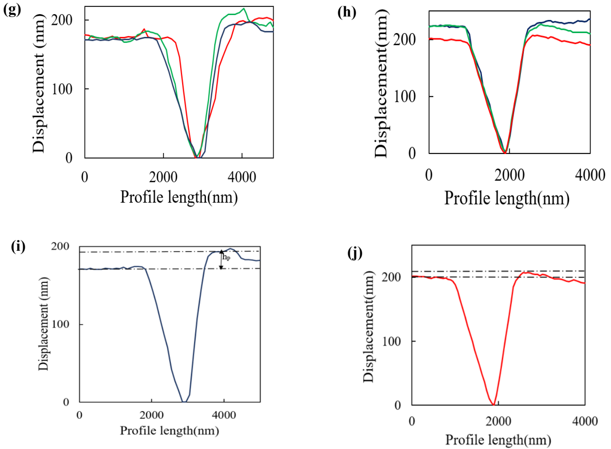
Fig. 10. (a) AFM image before indentation on \text{Cu}_A (size of the square box is 44.5 \times 44.5 \mu\text{m}^2 ); (b) AFM image before indentation on \text{Cu}_A/\text{Gr} (size of the square box is 44.5 \times 44.5 \mu\text{m}^2 ); (c) AFM image after indentation on \text{Cu}_A (size of the square box is 25 \times 25 \mu\text{m}^2 ); (d) AFM image after indentation on \text{Cu}_A/\text{Gr} (size of the square box is 25 \times 25 \mu\text{m}^2 ); (e) Higher magnification of one indent on \text{Cu}_A ; (f) Higher magnification on one indent on \text{Cu}_A/\text{Gr} ; \text{Cu}_A ; (g) Three height profiles across the indent shown in (e); (h) Three height profiles across the indent shown in (f); (i) Height profile (dark blue) across the indent shown in (e); (j) Height profile (red) across the indent shown in (f).
