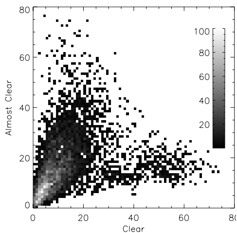
Figure 4. Fraction of almost clear cases (optical thickness less than 0.2) as a function of the number of totally clear cases. This figure is based on the monthly means shown in Figures 1 and 2. The color scale range is arbitrary.
