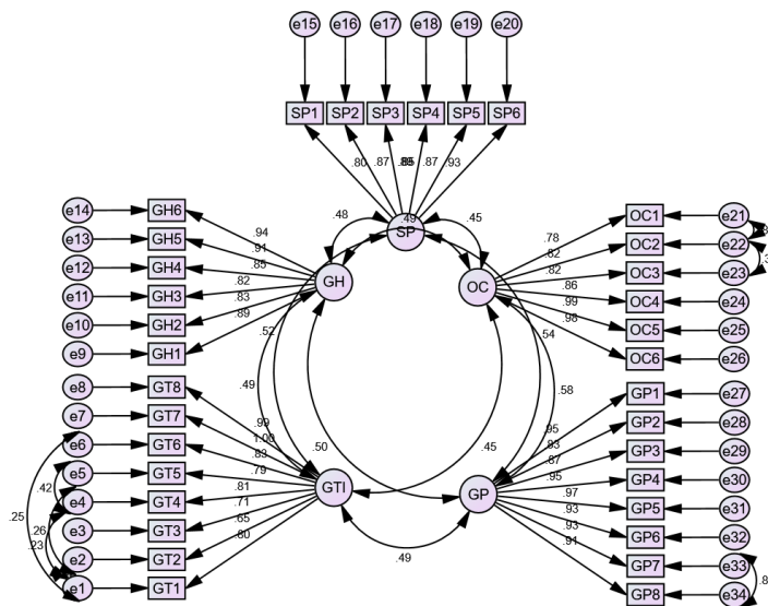
Figure 3: CFA
