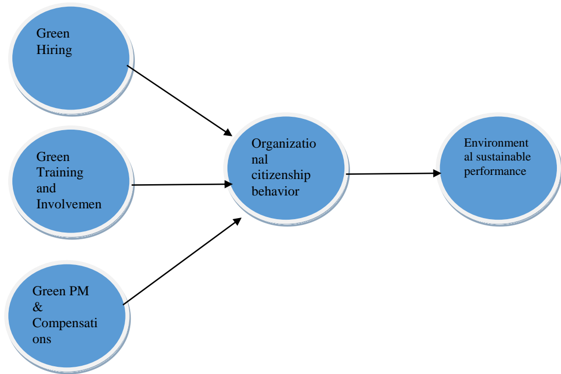
Figure 2: Research Model
