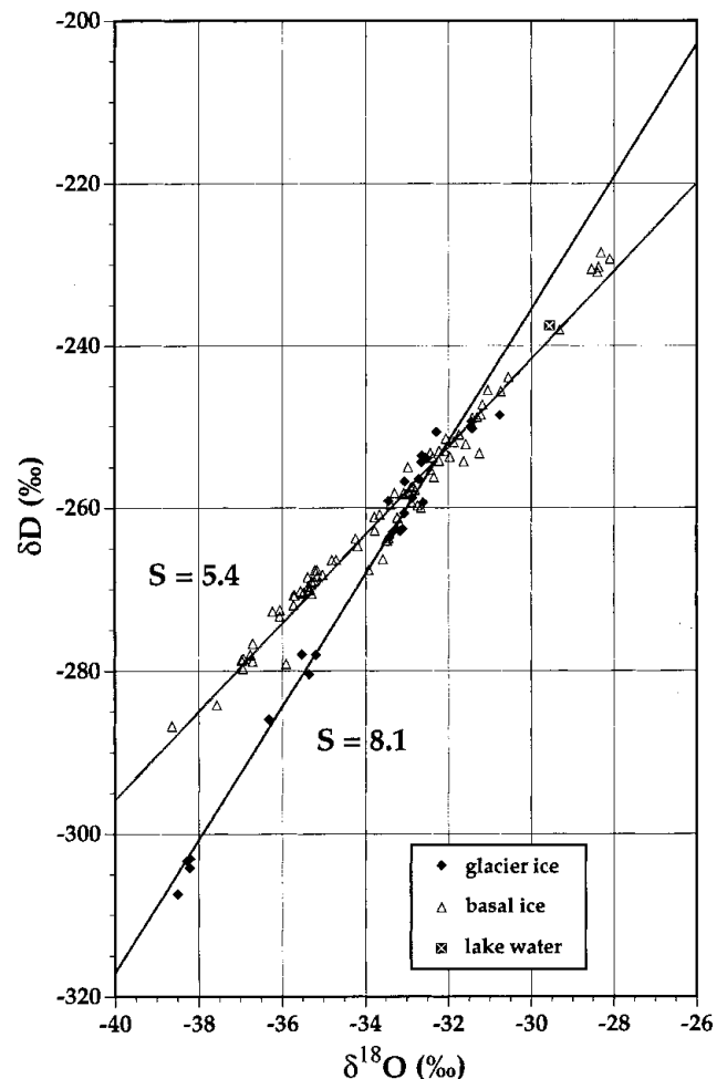
Fig. 6. \delta\text{D} – \delta^{18}\text{O} diagram of all samples analysed from: the glacier surface ( \blacklozenge ), from the basal ice ( \triangle ) of Sues Glacier; and from the lake water of Lake Popplewell ( \boxtimes ). S is the value of the slope of the nearby regression line.
