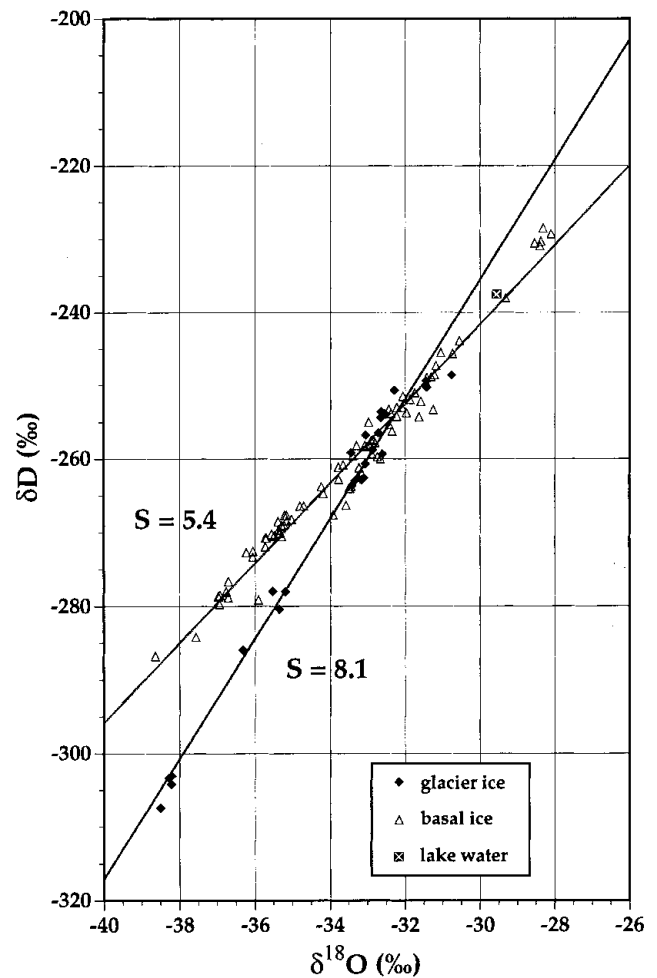
Fig. 6. \delta\text{D} – \delta^{18}\text{O} diagram of all samples analysed from: the glacier surface ( \blacklozenge ) from the basal ice ( \triangle ) of Sues Glacier; and from the lake water of Lake Popplewell ( \boxtimes ). S is the value of the slope of the nearby regression line.
