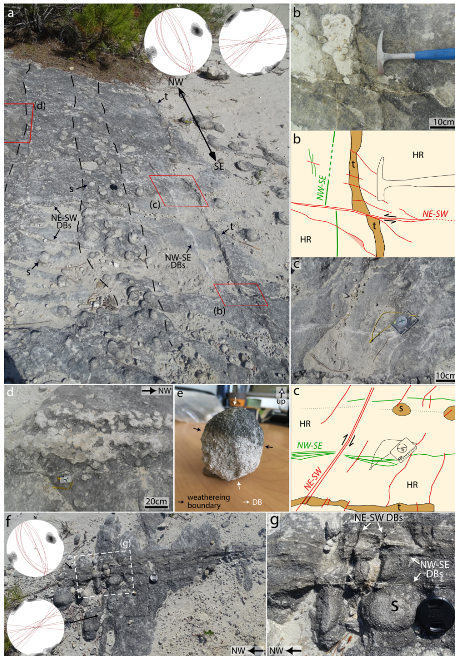
Figure 7. Calcite cement occurs isolated ( a, c, g ) or in clusters ( a, d ) of (S) spherical nodules and continuous (t) tabular nodules ( a–c ). Nodules are arranged in compartments parallel to clusters of NW–SE normal bands ( a–c ) and to NNW–SSE dextral strike-slip bands ( f, g ). NE–SW/ENE–WSW strike-slip bands displace both the NW–SE bands and their associated nodules ( a–c, f ). (e) Spherical nodule (about 5 cm in diameter) in spatial superposition with a NW–SE DB that does not displace the cement. The lens cover in ( a, f ) has a 5.5 cm diameter. The figures ( a–d, f, g ) are in map view. The position of ( a, f ) is indicated in Fig. 6b. Hammer length in ( b ) is 30.5 cm.
