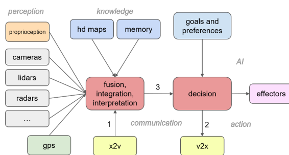
Figure 7: Diagram of modules which compound a connected and autonomous vehicle.
