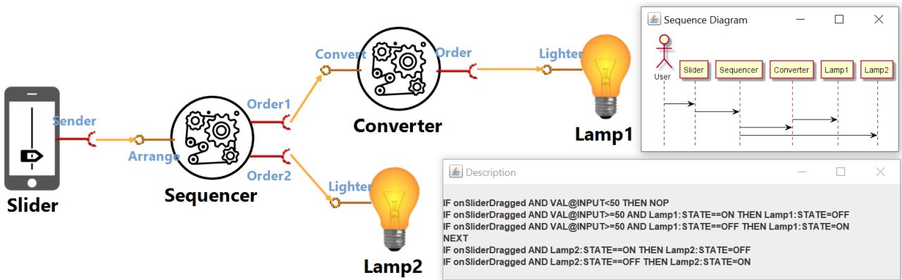
Figure 5.1: The parallel ambient lighting application
