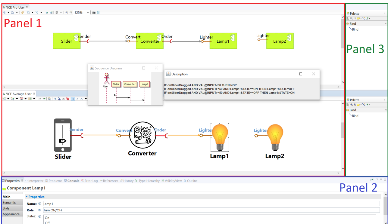
Figure 4.1: The Interactive Control Environment (ICE)
