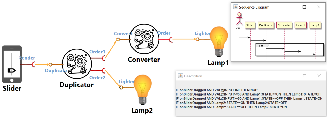
Figure 5.1: The parallel ambient lighting application
