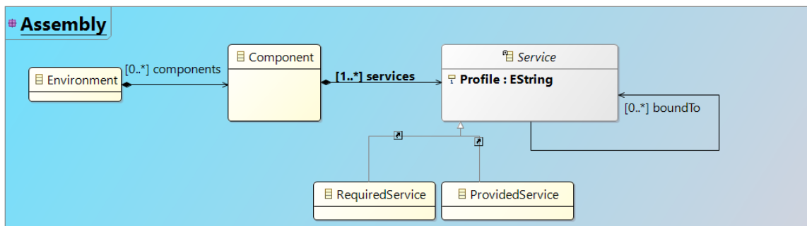
Figure 4.3: Assembly metamodel
