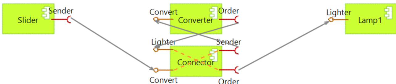
Figure 4.6: Connector-based assembly of the ambient lighting application
