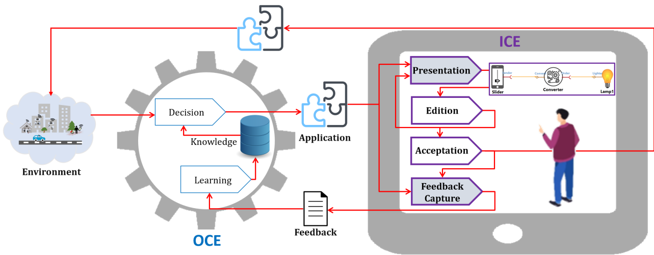
Figure 4.2: Overall architecture with the user in the loop
