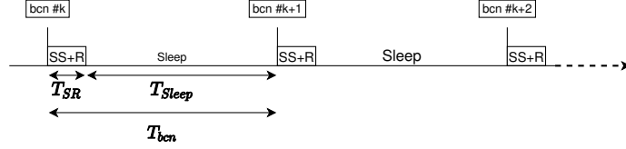
Figure 3: The behavior of the ENs during the SR operations: ENs wakes up for T_{SR} , then sleep till the next SR operation
