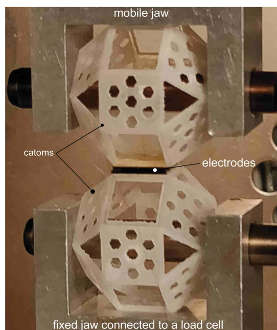
Figure 9. Experimental bench.
