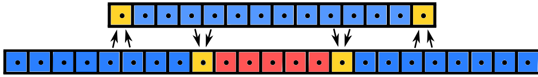
Figure 7. Scheme of an 1D overet mesh (top cell group) and its associated background mesh (bottom cell group). Blue cells are calculated, yellow cells are interpolated and red cells are disabled. The arrows represent the transfer of information from one mesh to another for interpolated cells.
