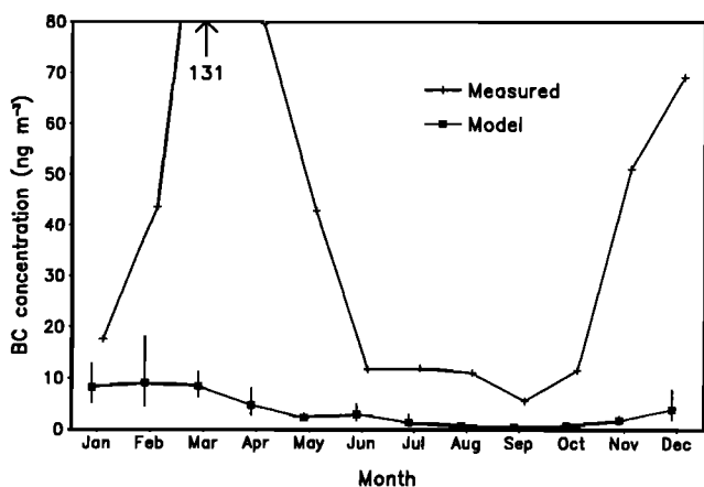
Figure 8. Comparison of modeled and measured black carbon at Barrow. Geometric deviations of the monthly means over the modeled period are shown.
