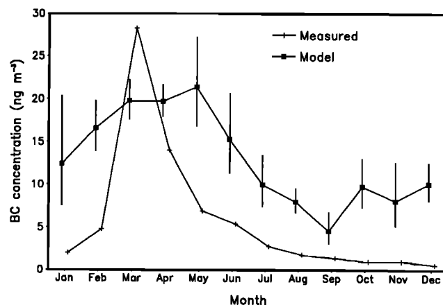
Figure 9. Comparison of modeled and measured black carbon at Mauna Loa. Geometric deviations of the monthly means over the modeled period are shown.
