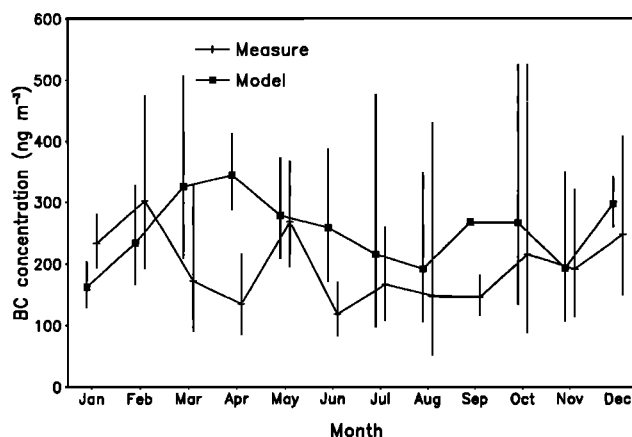
Figure 7. Comparison of modeled and measured black carbon at Mace Head for the continental sector. Geometric deviations of the monthly means over the measured and modeled periods are shown.
