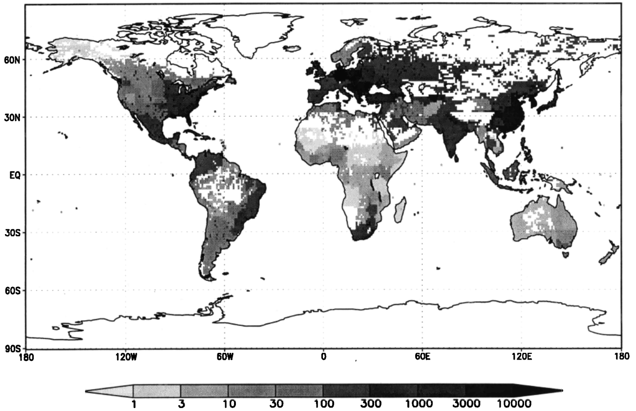
Figure 3. Global distribution of organic carbon (OC) emissions on a 1° x 1° scale.
