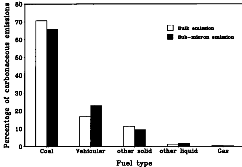
Figure 4. Relative contribution of various sources to global carbonaceous aerosol emission.
