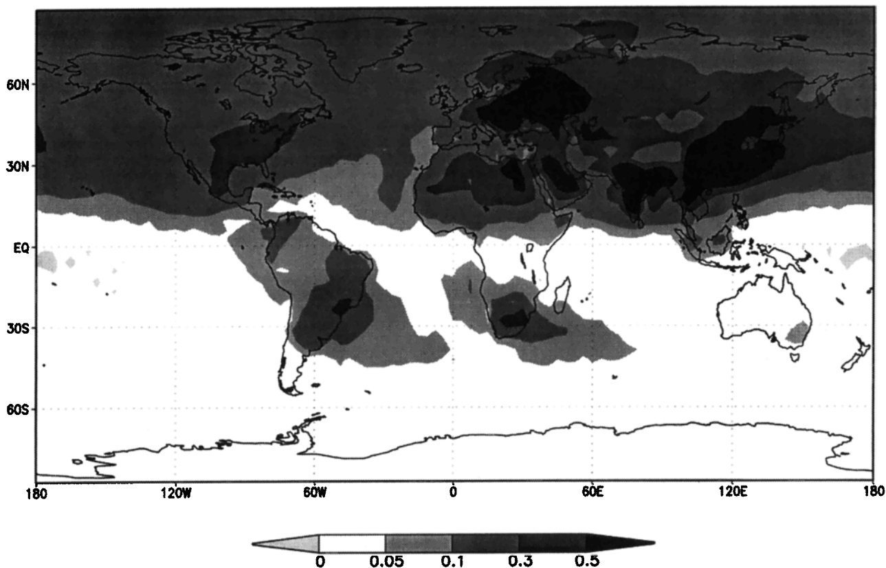
Figure 11. The annual average radiative forcing ( \text{W m}^{-2} ) due to BC and 2\times\text{OC} from fossil fuel combustion.
