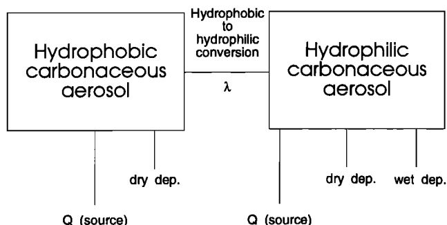
Figure 5. Emission and transformation scheme for carbonaceous aerosol.
