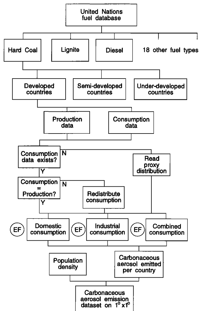
Figure 1. Tree diagram of emission distribution.
