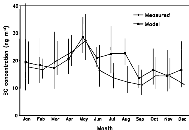
Figure 6. Comparison of modeled and measured black carbon at Mace Head for the marine sector. Geometric deviations of the monthly means over the measured and modeled periods are shown.
