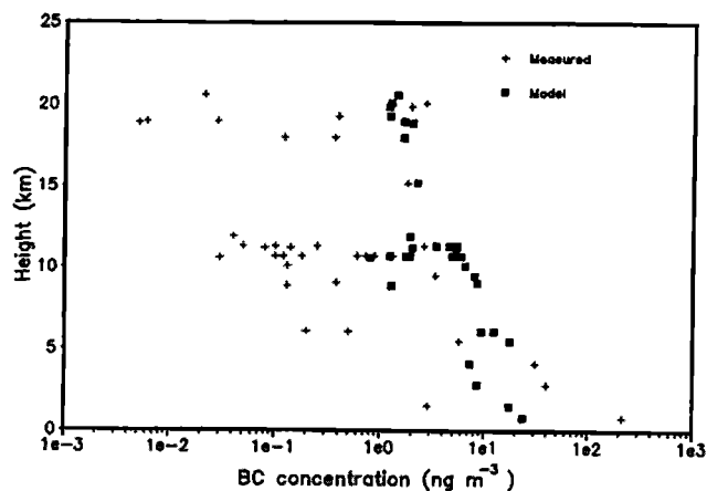
Figure 10. Comparison of BC vertical profile data.
