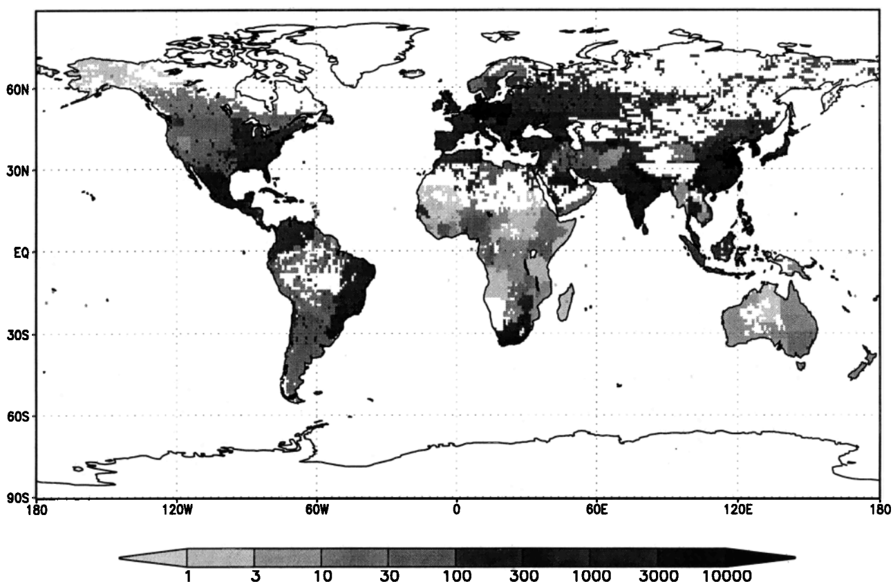
Figure 2. Global distribution of black carbon (BC) emissions on a 1° × 1° scale.
