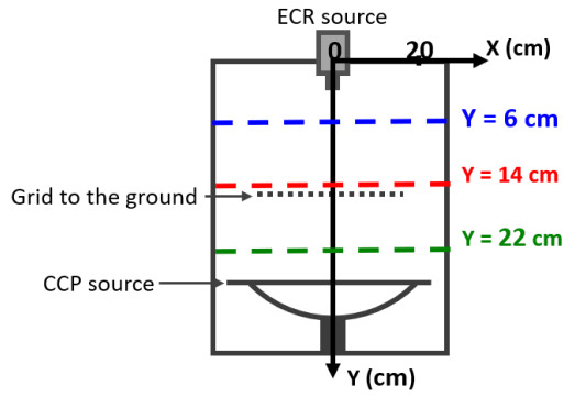
Fig. 2. Schematic diagram of the vacuum chamber and the plasma diagnostics positions.
