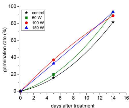
Fig. 8. Tomato seeds germination rates at 5 and 14 days after 10 min exposed to plasma – treatment power varied as indicated in legend.
