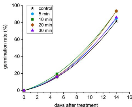
Fig. 7. Tomato seeds germination rates at 5 and 14 days after 50 W plasma treatments – treatment time varied as indicated in legend.
