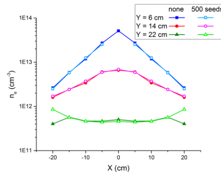
Fig. 6. Electron density radial distribution at 50 W without (full) and with (empty) seeds inside the reactor.
