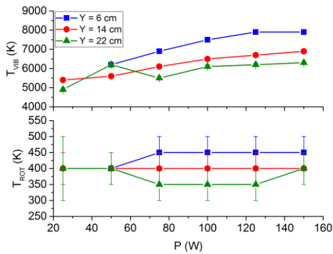
Fig. 3. T_{VIB} (top) and T_{ROT} (bottom) determined by the N_2(C - B) emission bands fitted with Specair software.
