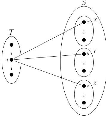
Figure 6: 3DMP bipartite graph H = (T, S, E')
