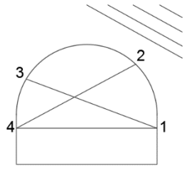
Fig13. Back analysis of convergence data of section 29 (chainage 2322) ( smallest convergence) and schematic average distribution of the targets (right) in the section (a) back analysis of convergence data of section 12 (chainage 1976) (largest convergence) and schematic average position of the targets (right) in the section (b)
