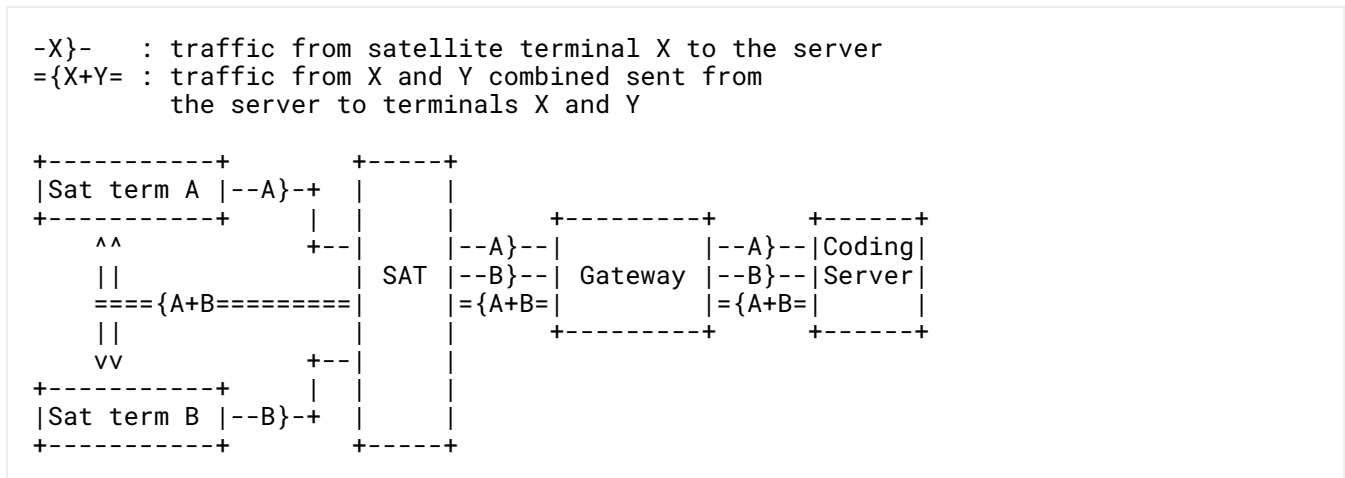
Figure 2: Network Architecture for Two-Way Relay Channel Using Network Coding
