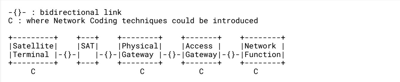
Figure 6: Network Architecture for Dealing with Varying Link Characteristics
