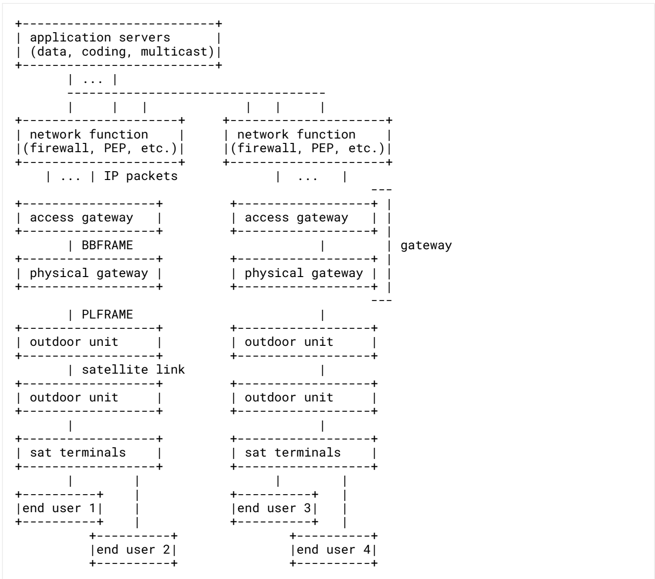
Figure 1: Data-Plane Functions in a Generic Satellite Multigateway System
