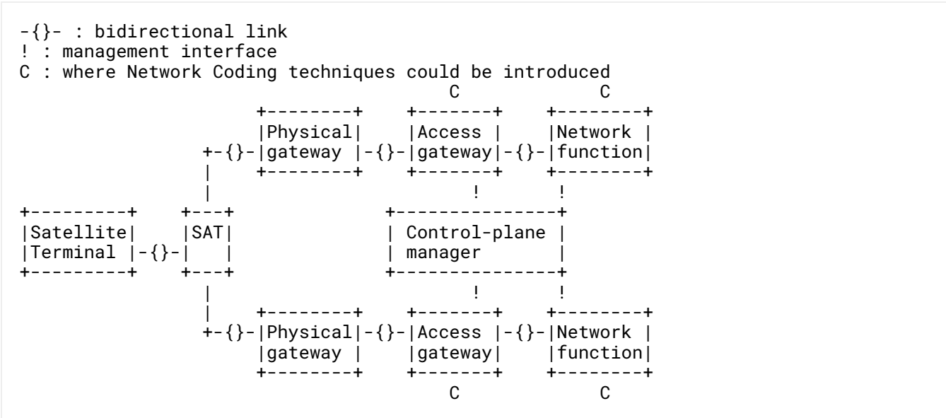
Figure 7: Network Architecture for Dealing with Gateway Handover
