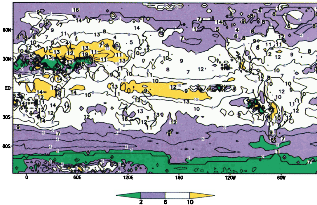
Plate 3. Annual mean of the deuterium excess (in per mil) in precipitation simulated by the ECHAM3 model (5 years T42-control) and observations from IAEA stations [IAEA, 1992]. The bold numbers give the long term means of the IAEA stations.
