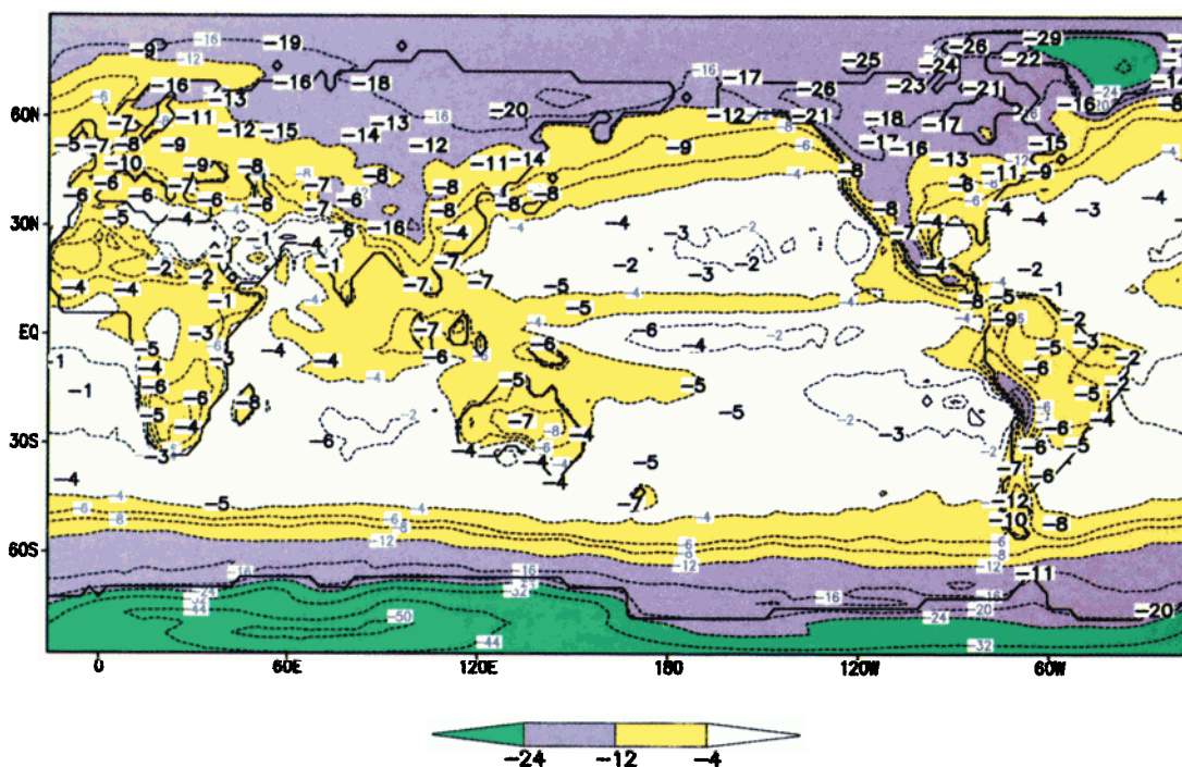
Plate 2. Seasonal cycle of \delta^{18}\text{O} in precipitation (in per mil) defined as DJF-JJA values simulated by the ECHAM3 (5 years T42-control) model and IAEA observations. The bold numbers give the seasonal amplitude of IAEA stations with at least three seasonal cycles.
