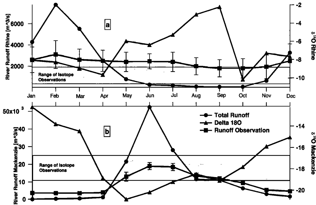
Figure 6. ECHAM3 T42-control and observations: River runoff (in \text{m}^3/\text{s} ) and its isotopic composition (in per mil) of the rivers (a) Rhine and (b) Mackenzie (the observations of the runoff are from the Global Runoff Data Center (GRDC) network [Dümenil et al. , 1993], the observed range of isotope observations is taken from Fritz [1981] and Hitchon and Krouse [1972]). For details of the calculation of the runoff see the Appendix.
