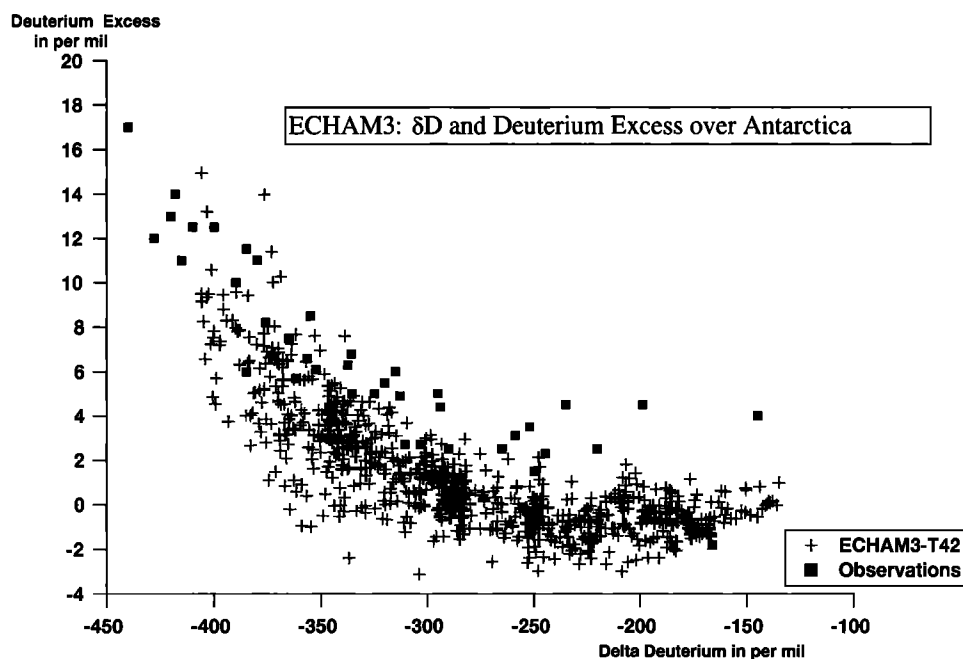
Figure 7. Deuterium excess d in precipitation over Antarctica versus the corresponding \delta D values simulated by the ECHAM3 T42-control run over 5 years (the pluses represent all grid point results over Antarctica). The observations (squares) are adapted from Petit et al. [1991].
