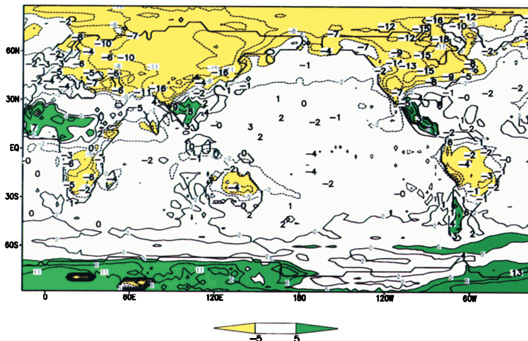
Plate 1. Annual mean of \delta^{18}\text{O} in precipitation (in per mil) simulated by the ECHAM3 model (5 years T42-control) and IAEA station data [IAEA, 1992]. The bold numbers give the long-term means of the IAEA stations.
