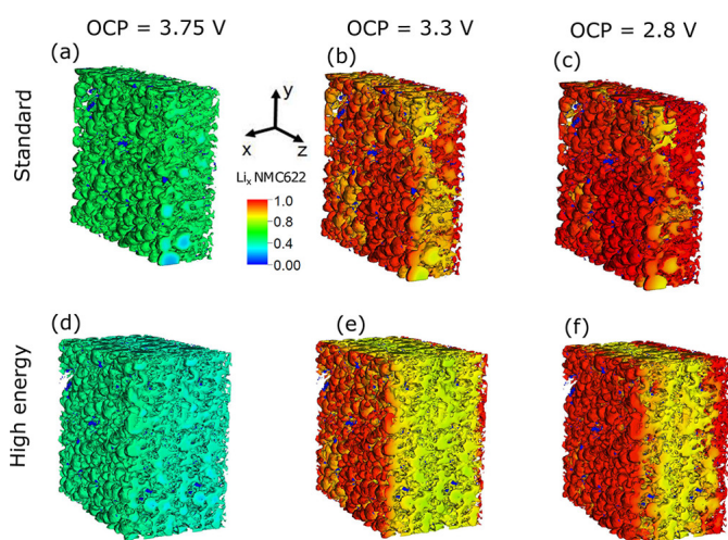
Figure 6. (a–c) Lithium distribution in the active material of the standard composite cathode (40 μm) at cell voltages of 3.75, 3.3, and 2.8 V during a 0.1C discharge. (d–f) Concentration distributions in the high-energy cathode (80 μm) under the same conditions. Reprinted from ref. 67 . Copyright (2020) American Chemical Society.
