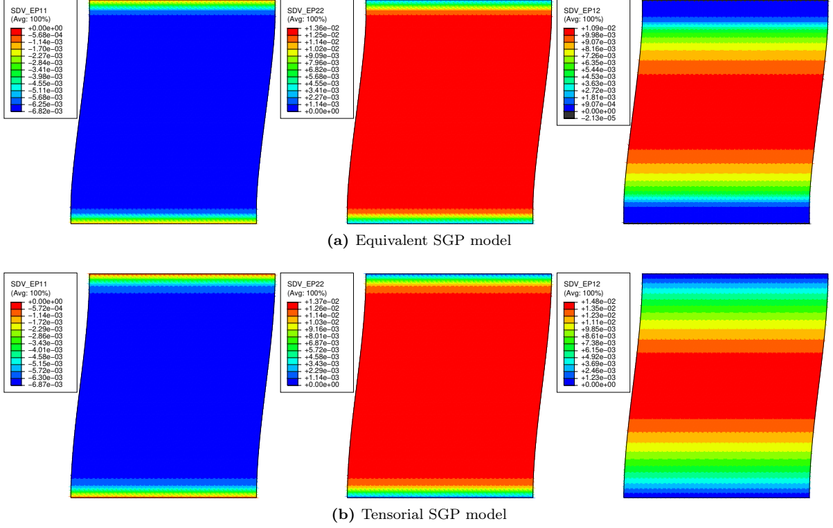
Figure 11: Distributions of plastic strain components within the studied plate, obtained using imposed tensile strain \varepsilon = 2\gamma = 0.02 and l/w = 0.4
