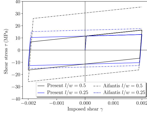
Figure 8: Cyclic shear results obtained using the present and the Aifantis theories for different values of l
