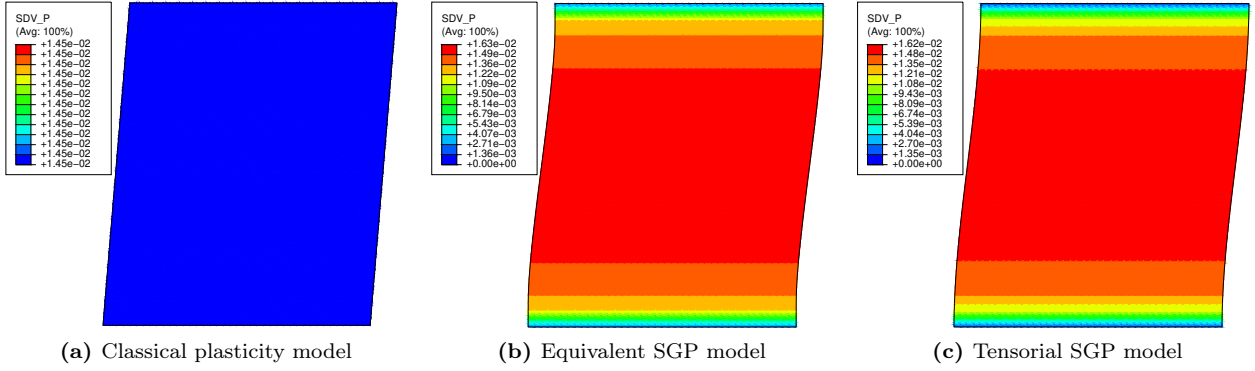
Figure 10: Distribution of cumulative plastic strain within the studied plate, obtained using imposed tensile strain \varepsilon = 2\gamma = 0.02 and l/w = 0.4
