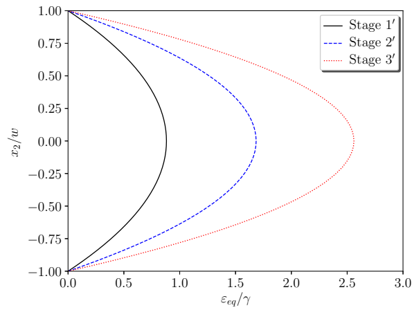
(c) Cumulative plastic strain profiles at stages 1' to 3' of figure 9a, obtained using the Aifantis model
