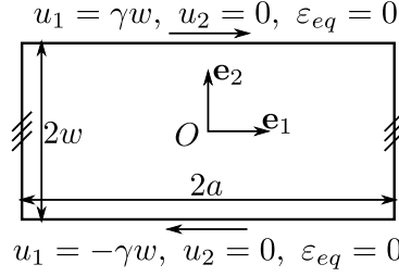
Figure 2: 2D strip subjected to simple shear loading and vanishing plastic stain on the top and bottom edges
