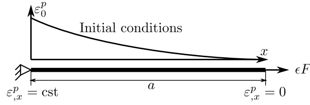
Figure 1: One-dimensional model subjected to initial conditions \varepsilon_0^p and a small perturbation \epsilon F , of which the direction is determined by the sign of \epsilon .
