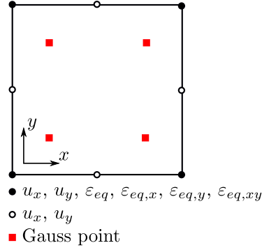
Figure 4: C^1 – continuous element
