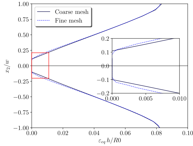
Figure 7: Effects of the mesh refinement on the plastic strain distributions in the vicinity of the neutral axis for \kappa = 3.67 \times 10^{-2} \text{ mm}^{-1}
