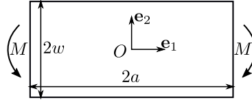
Figure 3: Thin foil subjected to simple bending loading and zero generalized traction on the top and bottom edges
