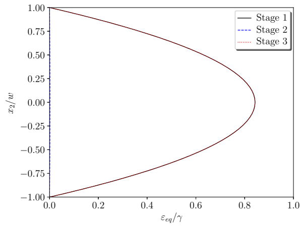
(b) Equivalent plastic strain profiles at stages 1 to 3 of figure 9a, obtained using the proposed model
