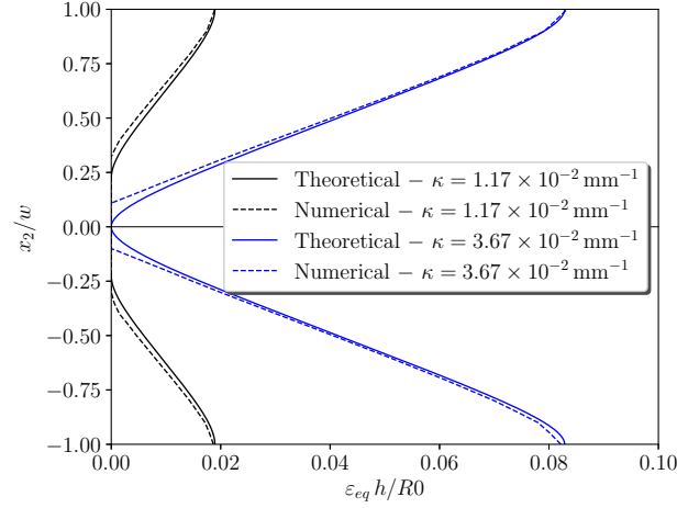
Figure 6: Equivalent plastic strain profiles along \mathbf{e}_2 -direction at different imposed curvatures
