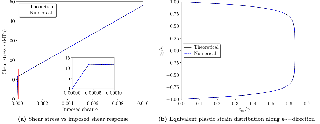
Figure 5: Simple shear results obtained using the present model
