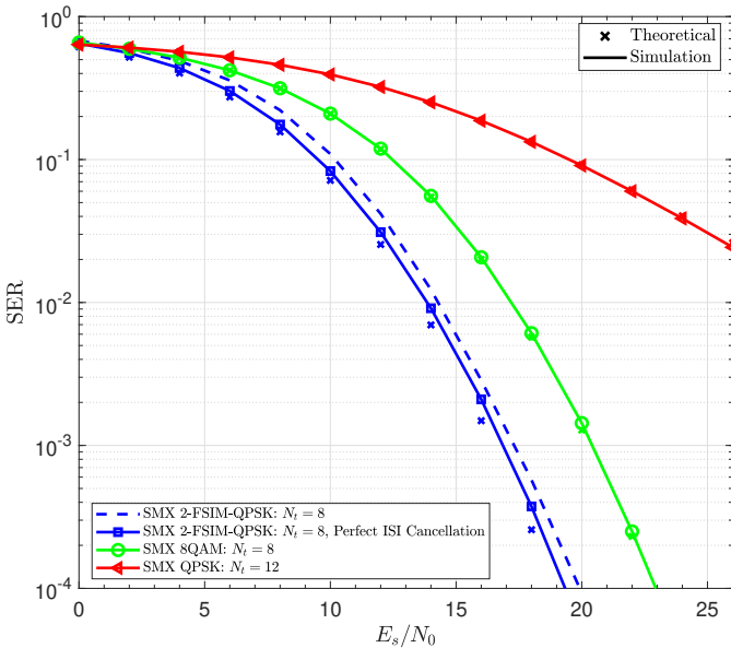
Fig. 5. SER performance of the proposed SMX 2-FSIM-QPSK system and its equivalent SMX-QAM systems of same SE= 24 bpcu and N_r = 12 .
