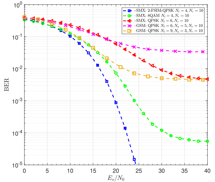
Fig. 11. Un-coded BER performance of the proposed non-coherent SMX FSIM compared to SMX-QAM and GSM in sub-THz channels with medium phase noise ( \sigma_g^2 = 10^{-2} ). The SE for all systems is 12 bpcu.
