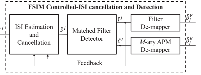
Fig. 3. System model of FSIM demodulator with the controlled-ISI cancellation and detection.
