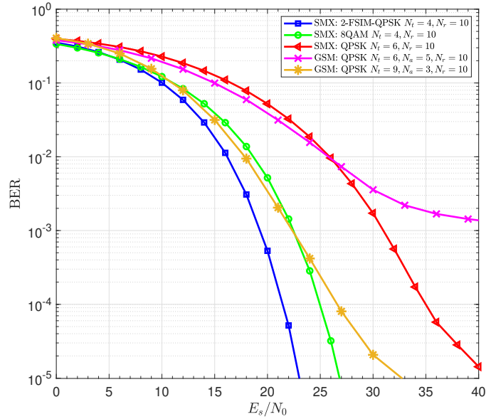
Fig. 10. Un-coded BER performance of the proposed non-coherent SMX FSIM compared to SMX-QAM and GSM in sub-THz channels with low phase noise ( \sigma_g^2 = 10^{-1} ). The SE for all systems is 12 bpcu.
