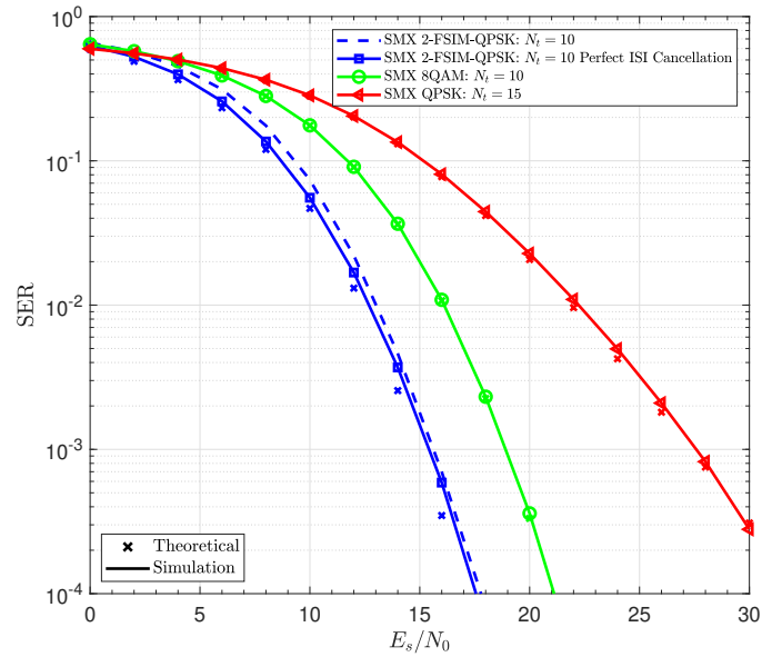
Fig. 6. SER performance of the proposed SMX 2-FSIM-QPSK system and its equivalent SMX-QAM systems of same SE= 30 bpcu and N_r = 16 .
