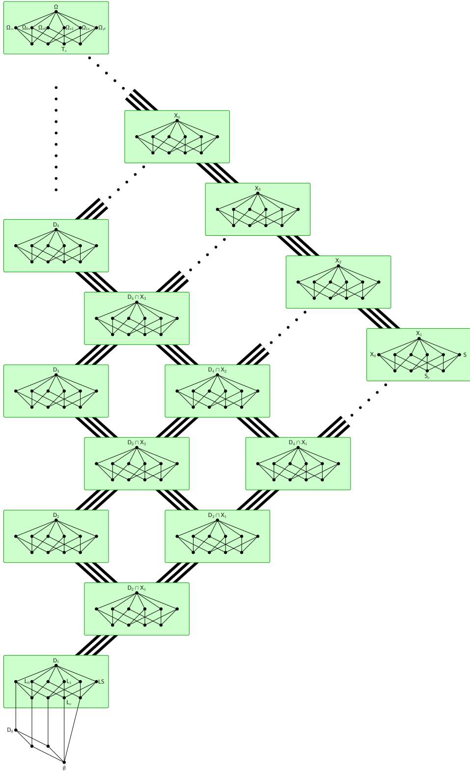
FIGURE 3. L_c -stable classes.
