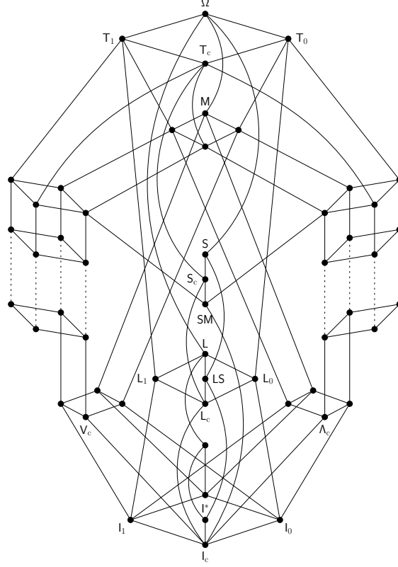
FIGURE 1. Post's lattice.
