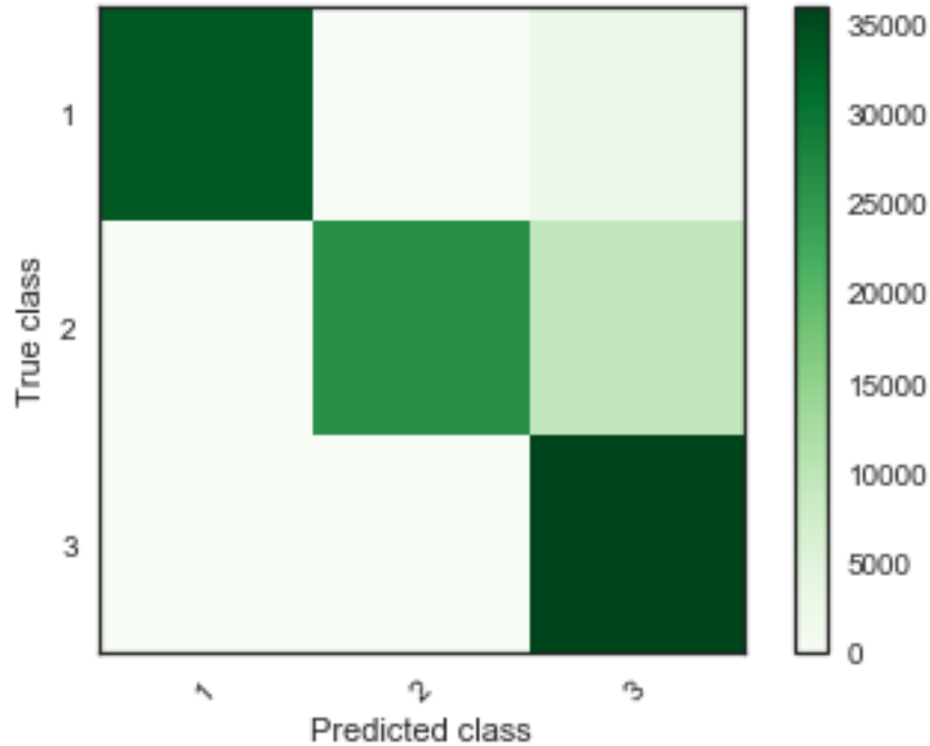
Figure 10. Confusion matrix for accident dataset
