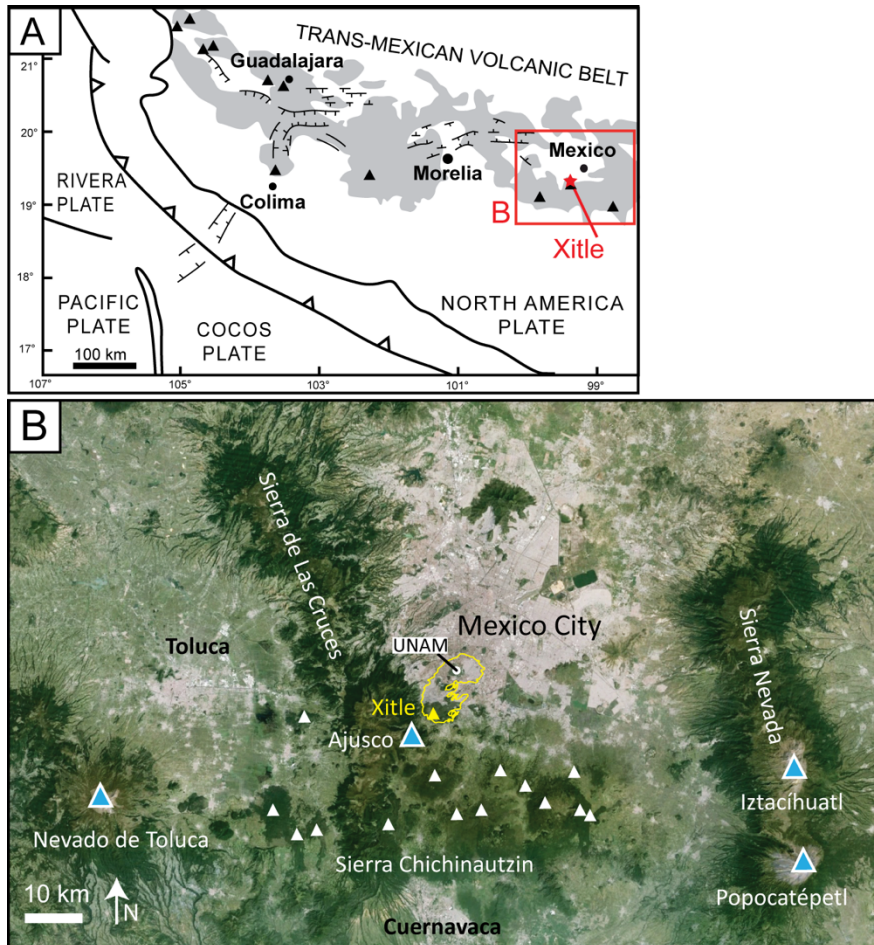
Fig. 1 A. Localization of the Xitle volcano and Mexico City in the Trans-Mexican Volcanic Belt and associated arc-type tectonic system. Dark filled triangles indicate mayor stratovolcanoes along the belt. Black filled points indicate main cities with millions of inhabitants. Note that most of these are located in the volcanic belt and hence at risks from new and ongoing eruptions. B. Localization of Xitle volcano (yellow triangle) and Xitle lava field (yellow polygon) including the UNAM campus, in the SW corner of the Mexico Basin host to Mexico City. White triangles are volcanoes of the Sierra Chichinautzin formed during the last 15,000 yrs. Blue and white triangles are stratovolcanoes. Popocatepetl is in eruption since 1994, while the Nevado de Toluca last erupted 10,000 yrs ago. Ajusco is extinct
