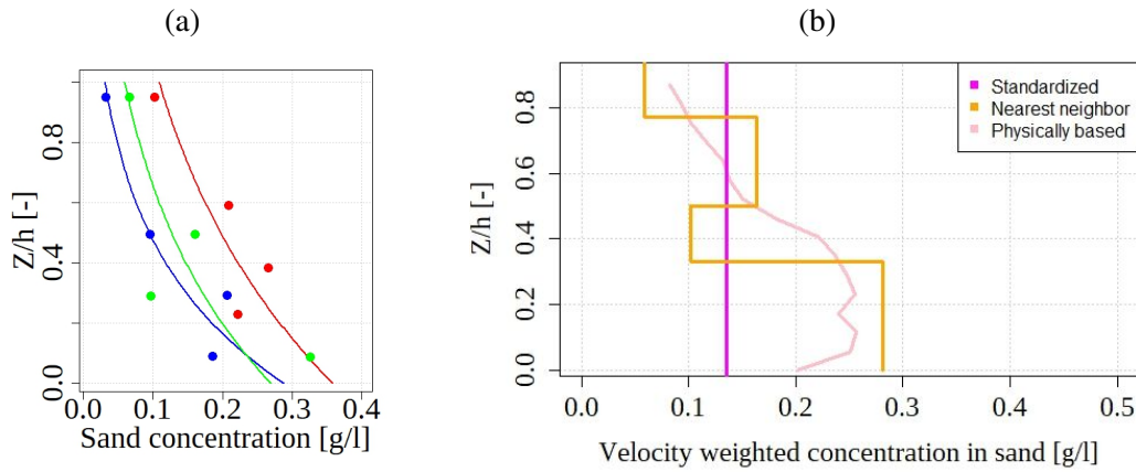
Figure 3. Exponential profile fitted on 3 verticals at Diamond Creek (04/01/2019) during suspended sand discharge measurement (a). One velocity weighted concentration vertical computed with 3 methods (b).
