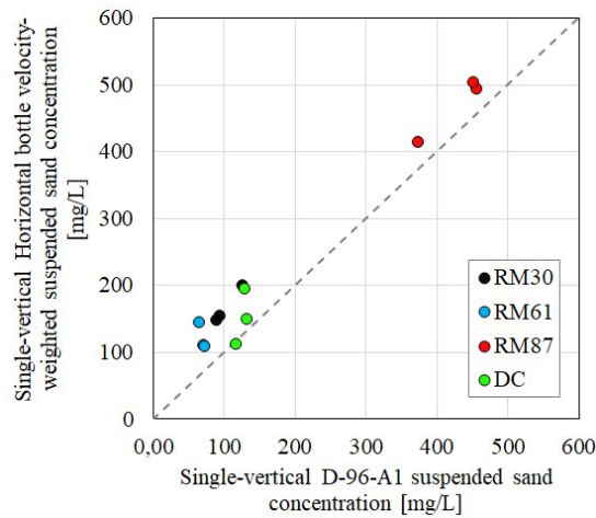
Figure 4. Single-vertical velocity-weighted sand concentrations from Van Dorn bottle compared to D-96-A1 sampler. Each point is one vertical comparison and each color belongs to the same cross section (with 3 different verticals).
