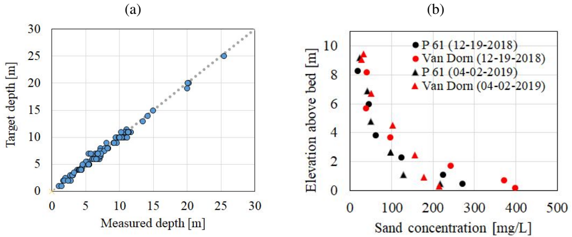
Figure 2. Depth sampling comparison between a pressure sensor and readings on the line by a field operator (a). Detailed vertical sand concentration profile at Diamond Creek, each concentration point is the average of three sample analysis (b).
