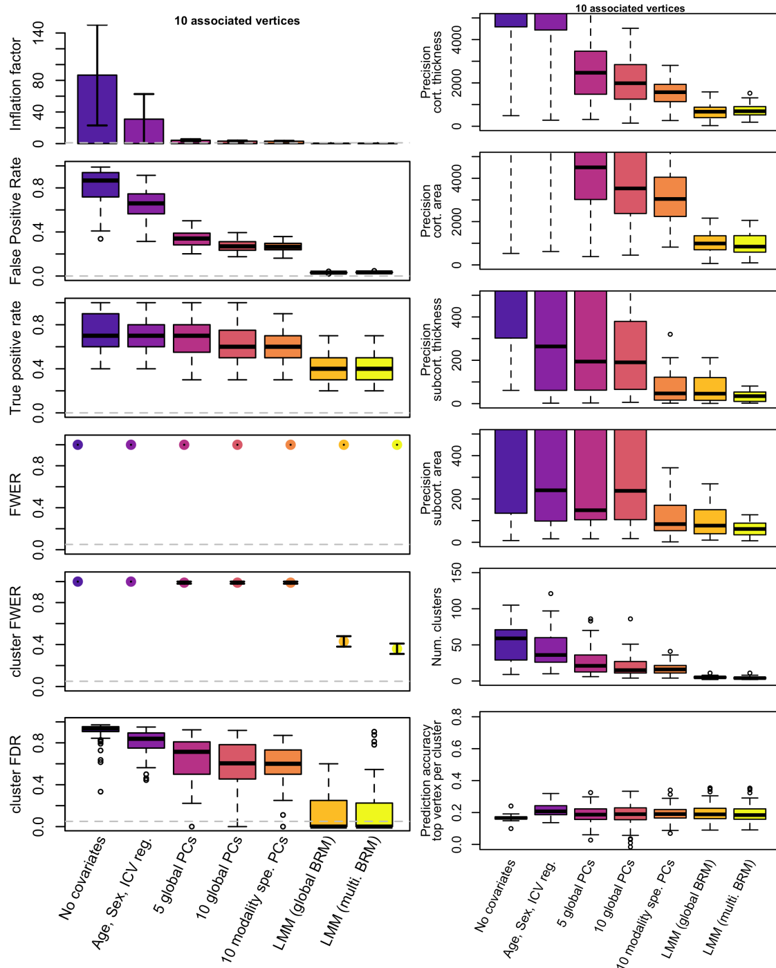
Figure 7: Results of mass-univariate analyses using smoothed meshes of cortical vertices.
