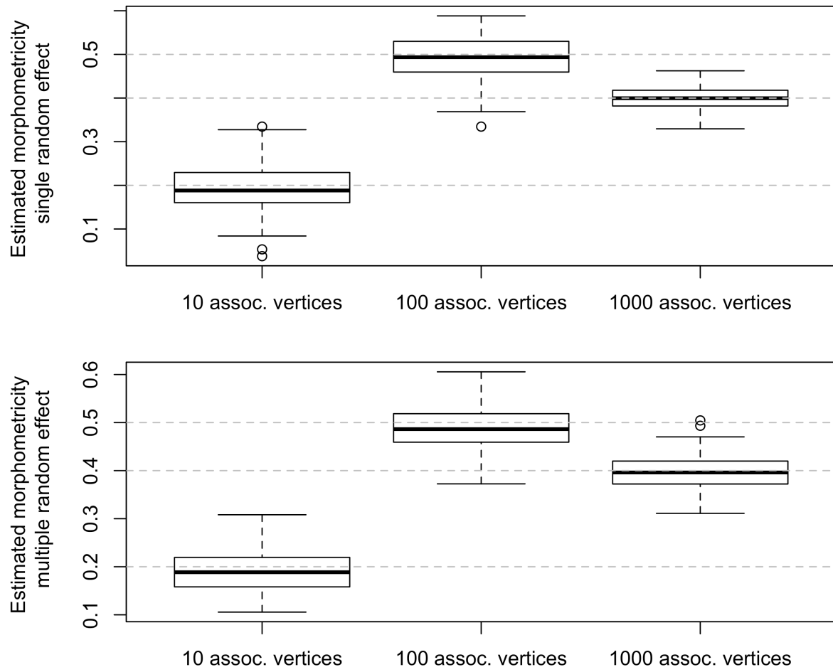
SFigure 8: Morphometricity estimates of our simulated traits from our two LMM models The grey lines represent the expected values.
