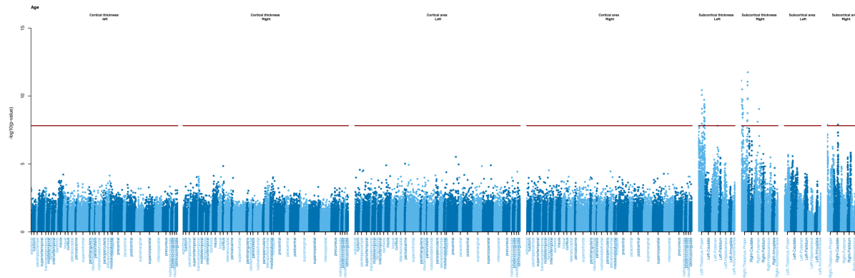
Figure 10: Manhattan plot of mass-univariate vertex-wise analysis of age
