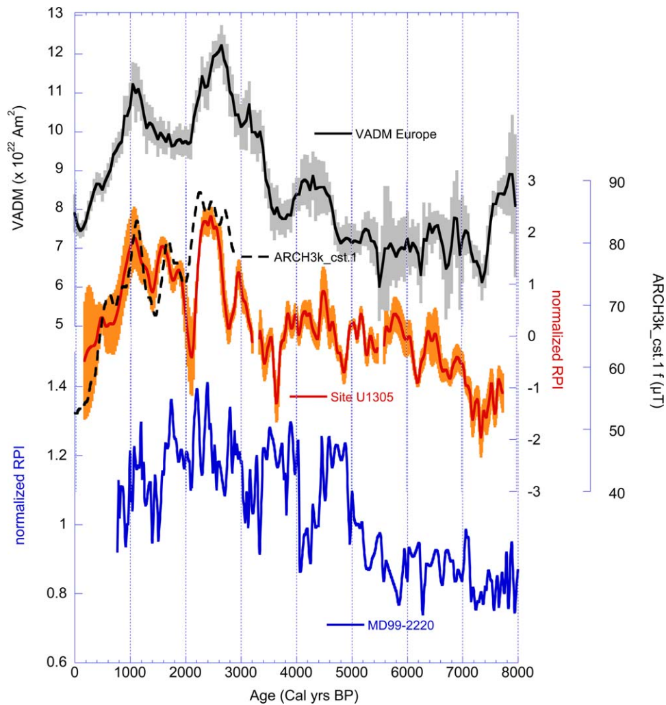
Figure 9. Paleointensity comparison across the North Atlantic. From top to bottom, the European archeomagnetic intensity compilation (black) [Genevey et al., 2008], RPI estimate for Site U1305 (red) as developed in Figure 4 on the tuned chronology in Figure 8, overlain by ARCH3k_cst.1 intensity predictions for the northern North Atlantic (black stippled) [Korte et al., 2009], and the RPI record from St Lawrence Estuary core MD99-2220 (blue) record [St-Onge et al., 2003].
