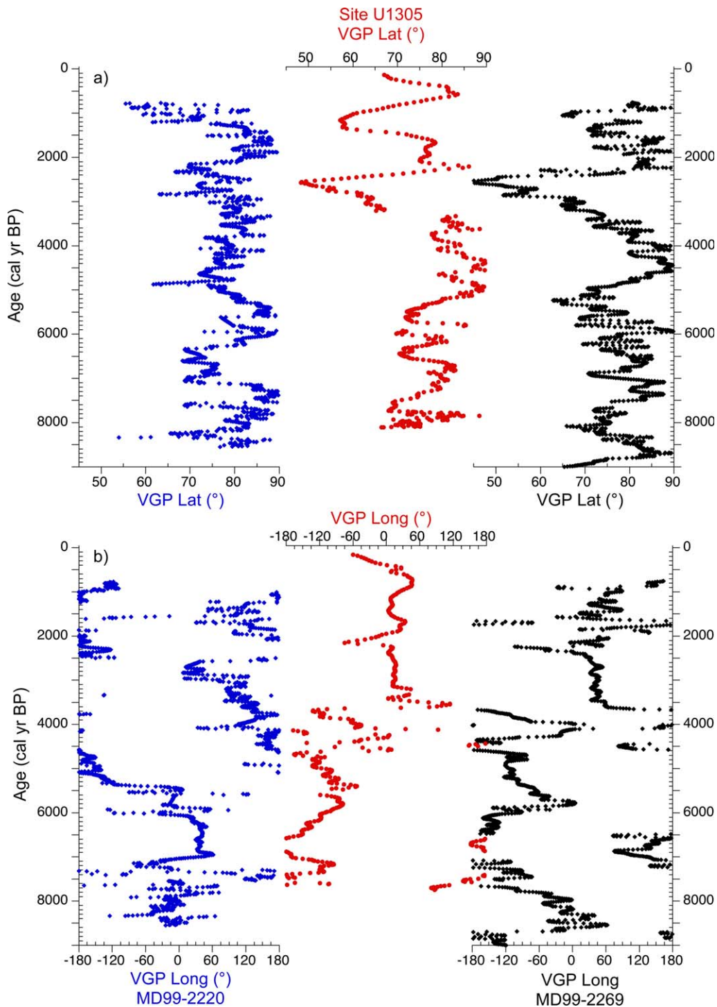
Figure 10. Comparison of PSV records expressed as virtual geomagnetic poles (VGP). (a) VGP latitude from left to right, core MD99-2220 (blue) [St-Onge et al., 2003], the upper 4.5 mcd of Site U1305 (red) on the tuned chronology as developed in Figure 8, and the Greenland/Iceland PSV composite (black). (b) VGP longitude from left to right, core MD99-2220 (blue) [St-Onge et al., 2003], the upper 4.5 mcd of Site U1305 (red) on the tuned chronology as developed in Figure 8, and the Greenland/Iceland PSV composite (black). For locations see Figure 1 and Table 1.
