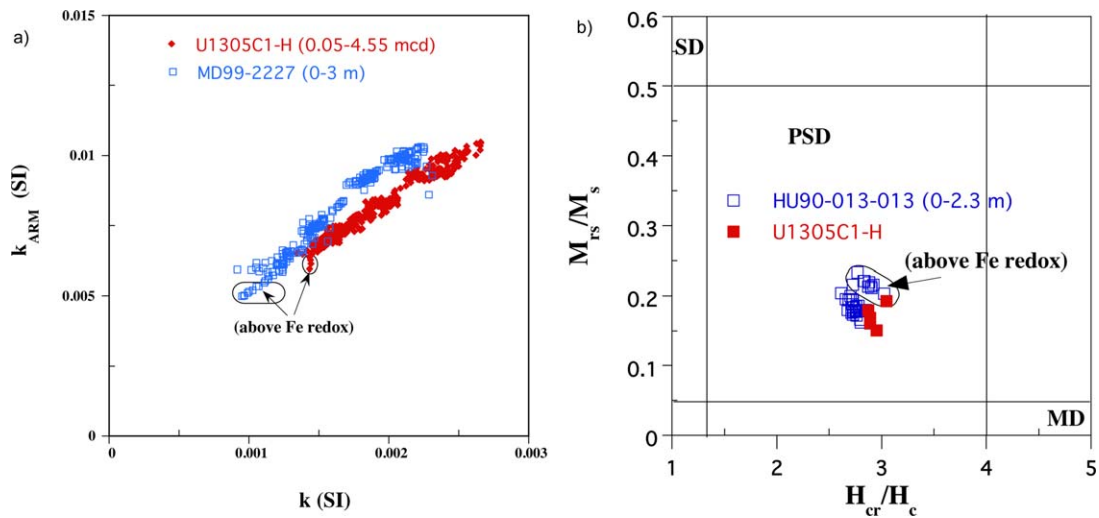
Figure 3. (a) Anhysteretic susceptibility ( \kappa_{ARM} ) plotted against susceptibility ( \kappa ) as a magnetic grain-size proxy after Banerjee et al. [1981] for the post-glacial sediments from the upper 4.5 mcd of Site U1305 compared with post-glacial sediments (upper 3 m) of Eirik Ridge core MD99-2227 [Evans et al., 2007]. (b) Magnetic hysteresis parameters ( M_{rs} , saturation remanence; M_s , saturation magnetization; H_{cr} , coercivity of remanence; H_c , coercive force) for the post-glacial sediments from the upper 4.5 mcd of Site U1305 compared with those from post-glacial sediments (upper 2.3 m) of Eirik Ridge core Hu90-013-013 [Stoner et al., 1995b]. Single domain (SD), pseudo-single domain (PSD), and multidomain (MD) fields are after Day et al. [1977]. Note: Cores MD99-2227 and Hu90-013-013 were collected from the same location. Sediments from above the Fe redox boundary ( \sim the upper 20 cm) are indicated. 4 mT was added to the H_{cr} values from Site U1305 to correct for differences assumed to result from the data being acquired on different instruments at different times.
