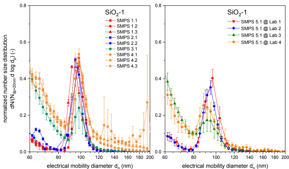
Fig2: Average particle number size distributions for the ERM-FD304 sample.
