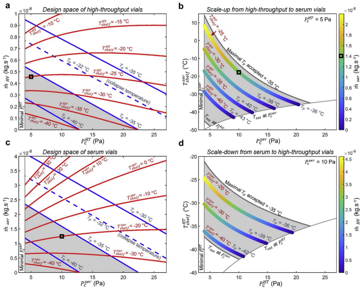
Figure 8 – Primary drying design spaces of a 5% sucrose solution calculated for: (a) high-throughput vials and (c) serum vials; and graphic solution to operate process change from: (b) high-throughput to serum vials, and (d) from serum to high-throughput vials. P_C^{HT} , T_{shelf}^{HT} , and \dot{m}_{HV} are the chamber pressure, shelf temperature and sublimation mass flow rate during primary drying performed with high-throughput vials, respectively. P_C^{ser} , T_{shelf}^{ser} , and \dot{m}_{ser} are the chamber pressure, shelf temperature and sublimation mass flow rate during primary drying performed with serum vials, respectively. T_{sat} is the ice-vapour equilibrium temperature. T_p is the product temperature, and the maximal T_p considered was -35\text{ }^\circ\text{C} . Blue lines in Figure 8a and Figure 8c represent iso- T_p curves and red lines iso- T_{shelf} curves. The grey area in the four graphs represents the safe zone of the process where T_p is lower than -35\text{ }^\circ\text{C} . Linear colour maps in (b) and (d) represent iso- T_p curves. Calculations were performed considering the global heat transfer coefficient between the shelf and the vial bottom for 500- \mu\text{L} vials in A-type well plates.
