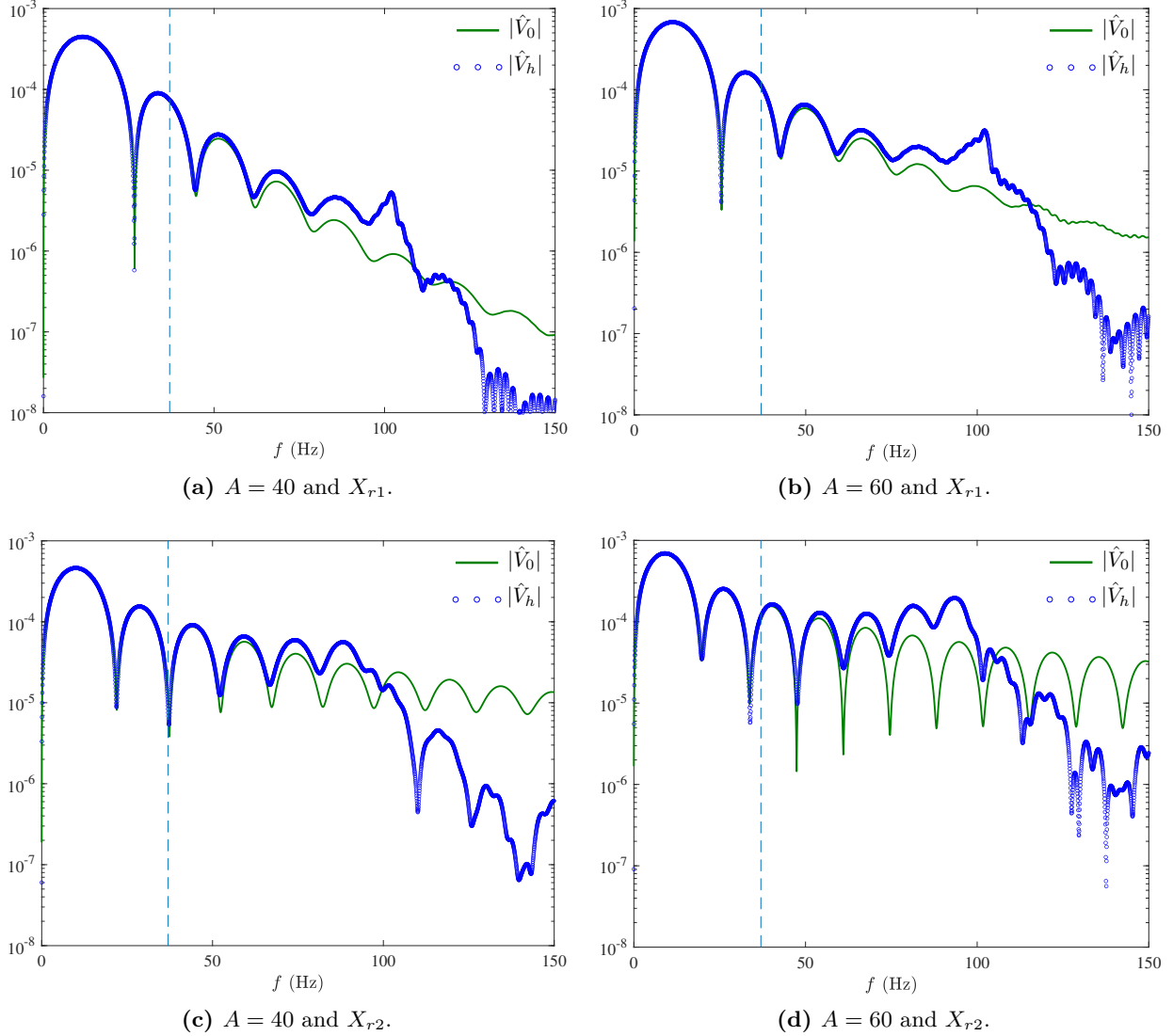
Figure 13: Case of a homogeneous periodic cell and an excitation by a pulse centered at f_c = 10 Hz with amplitude A = 40 (left panels) and A = 60 (right panels), as in Figure 12. Spectra of the velocity fields V_h and V_0 recorded at two receivers placed at X_{r1} = 1205 m and X_{r2} = 1705 m. The vertical dashed line indicates the value of the frequency that corresponds to \eta = 1 .
